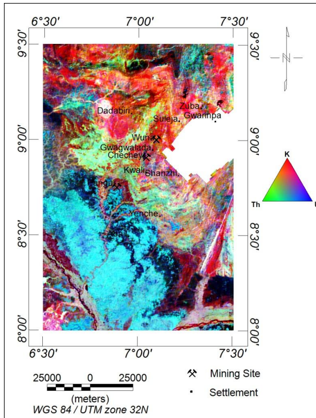
Figure 13. Ternary image of the study area
