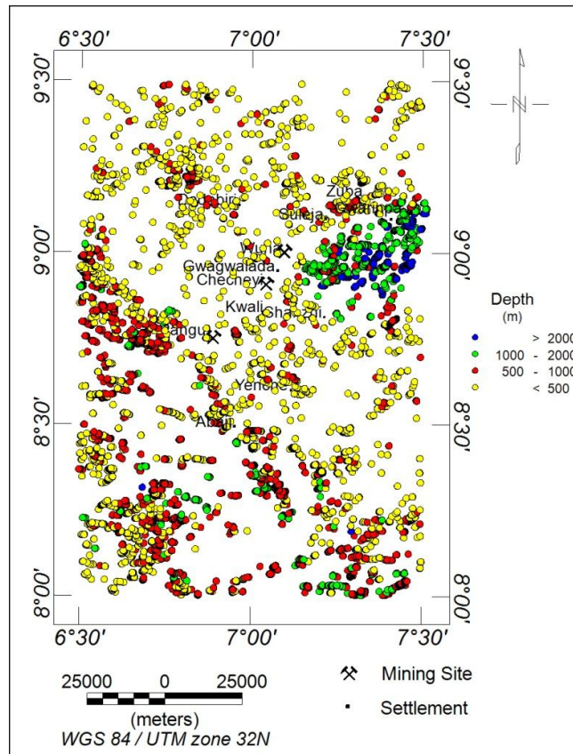
Figure 9. 3-D Euler depth solution
