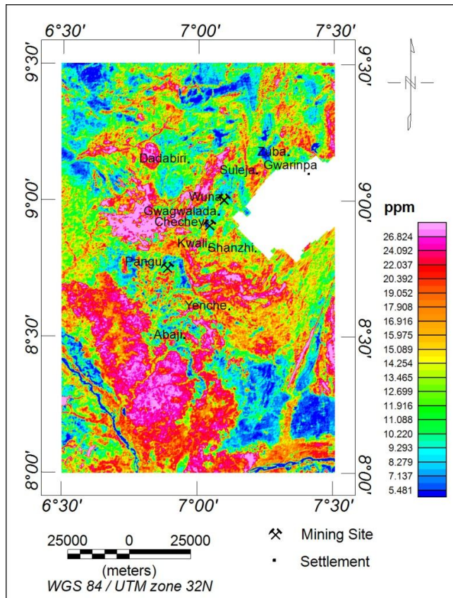
Figure 12. Equivalent Thorium (eTh) concentration map
