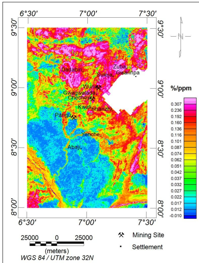
Figure 14. Potassium/Thorium ratio map of the study area
