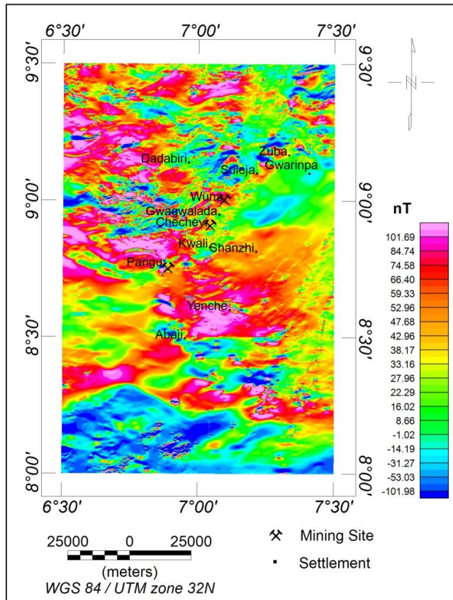
Figure 4. Reduced to the Equator map (RTE) of the study area
