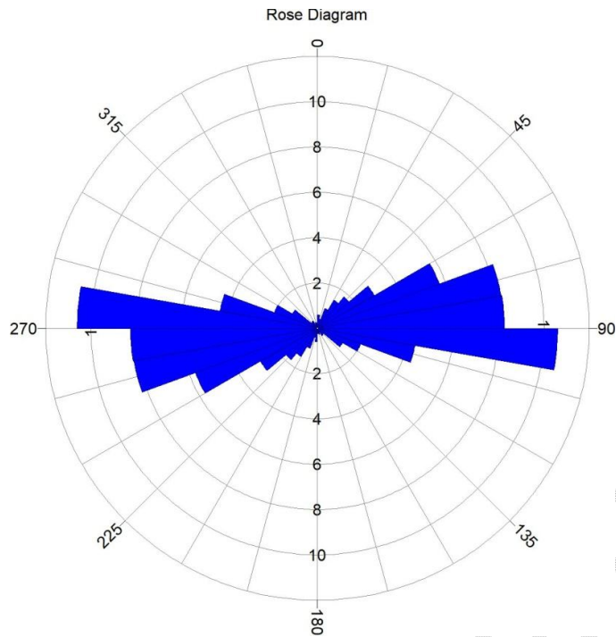
Figure 7b. Rose diagram showing the structural trending direction of the study area.
