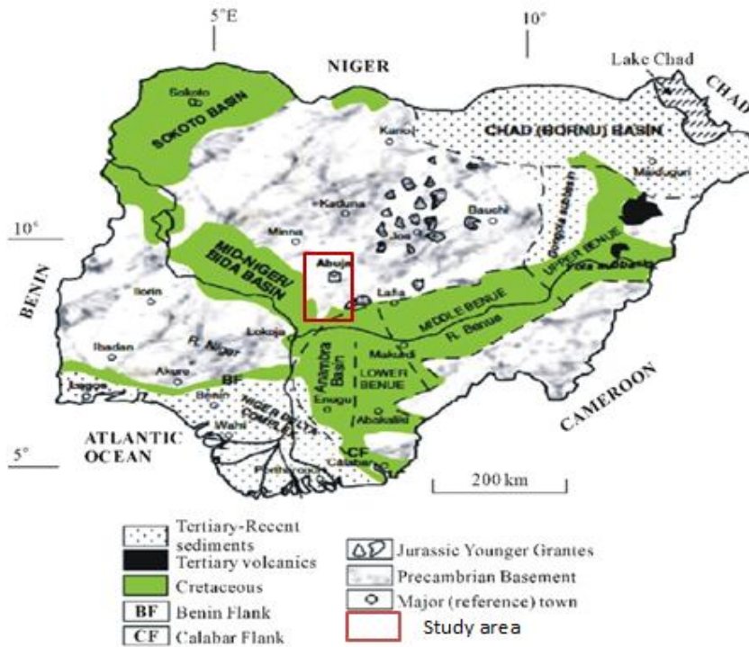
Figure 2. Geological map of Nigeria showing the study area and major geological components (modified after Obaje 2009).
