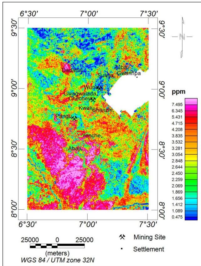
Figure 11. Equivalent Uranium concentration map
