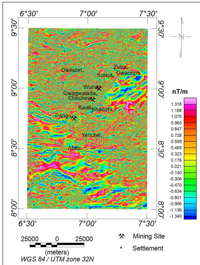
Figure 6. Tilt Derivative map of the study area
