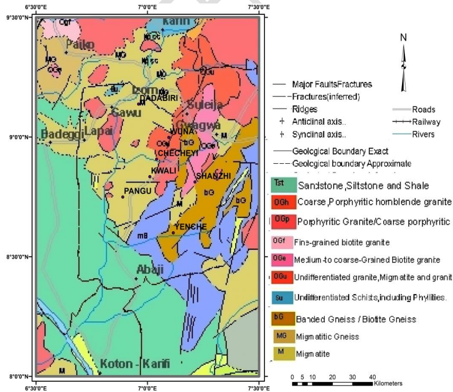
Figure 3. Geology map of the study area
