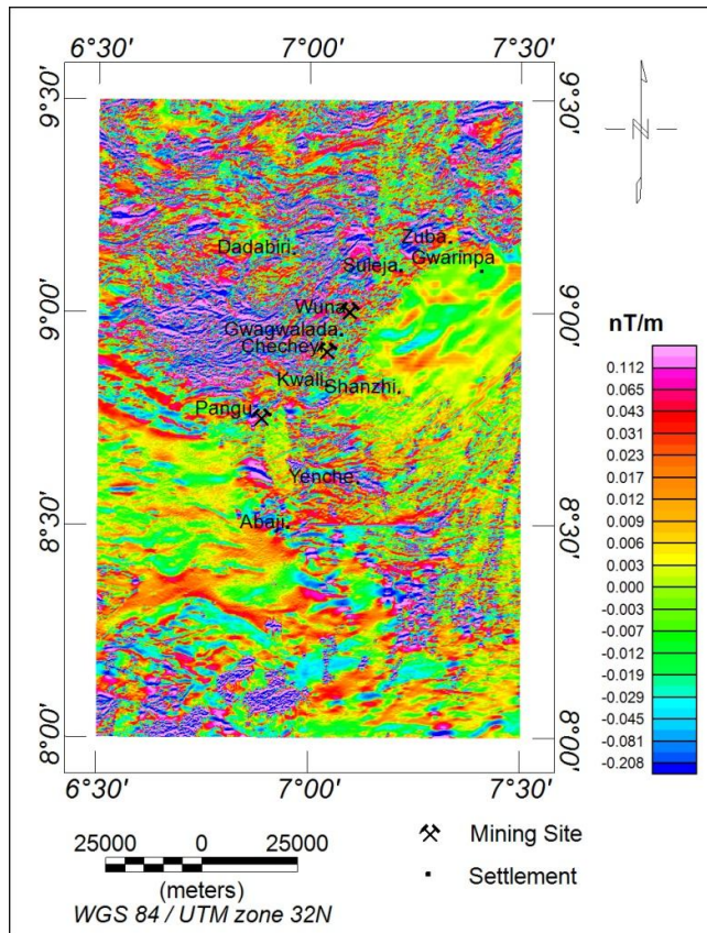
Figure 5. First Vertical Derivative map of the study area
