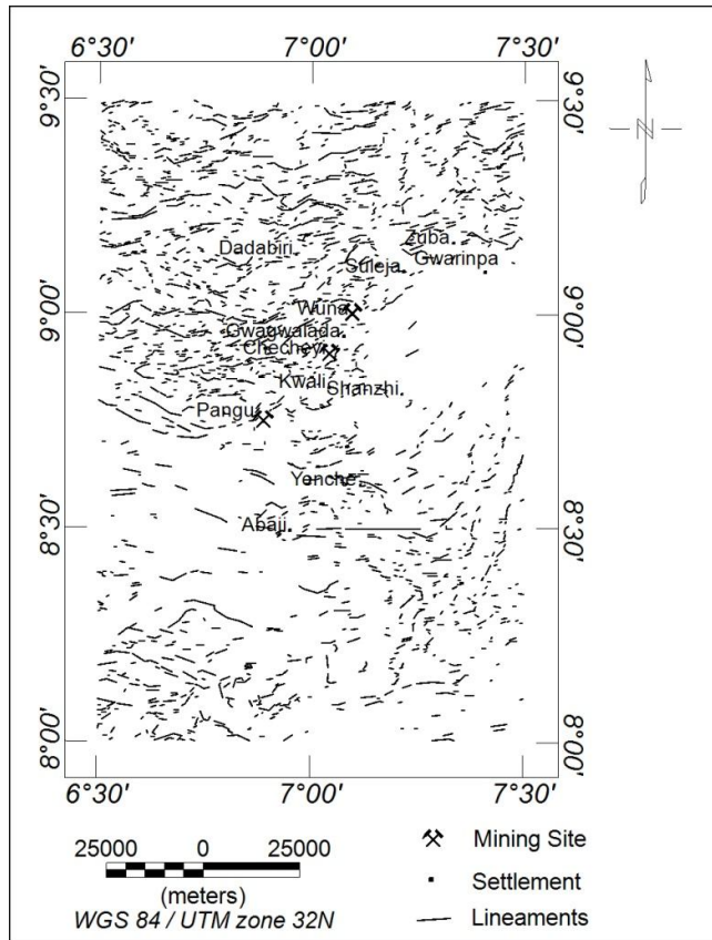
Figure 7a. Lineament map derived from CET grid analysis depicting faults
