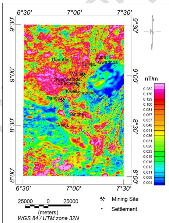
Figure 8. Analytic Signal map of the study area
