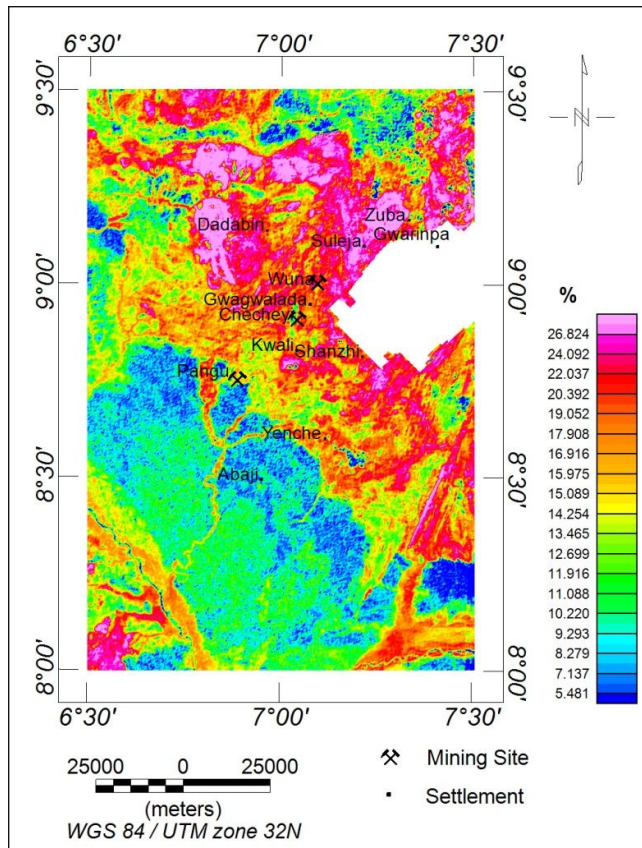
Figure 10. Potassium concentration map
