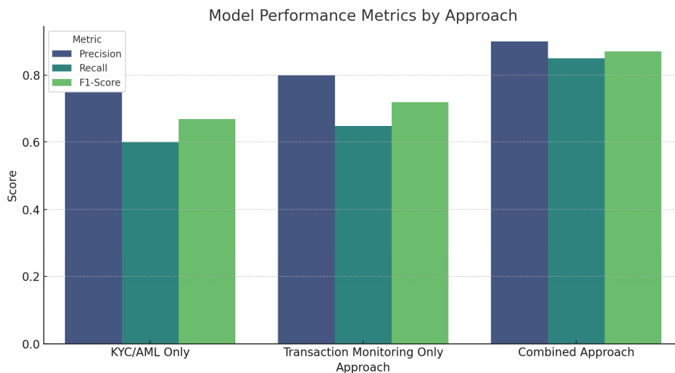
Figure 4 Model performance metrics by Approach
