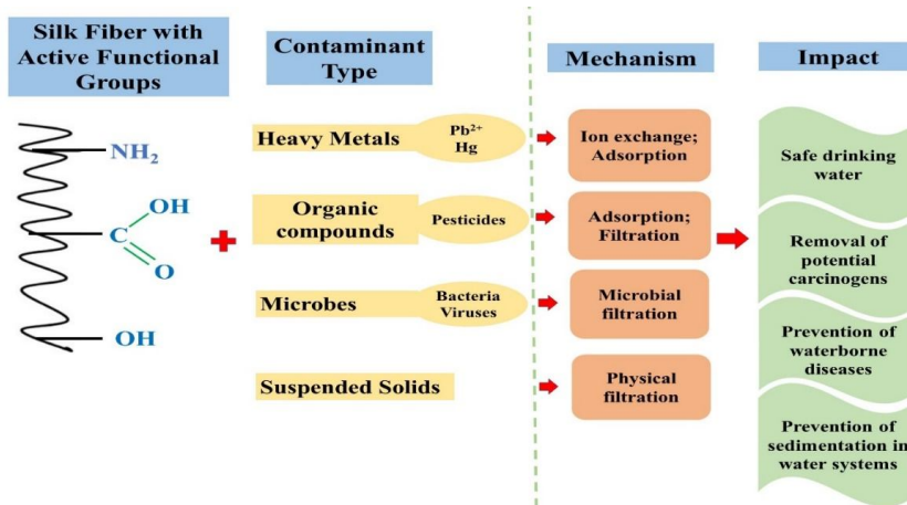
Fig.2 Mechanism of interaction between toxic contaminants and functional groups present on silk fibers
