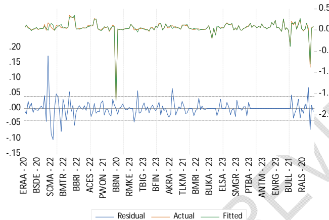
Fig2. Heterocedasticity Test Result
