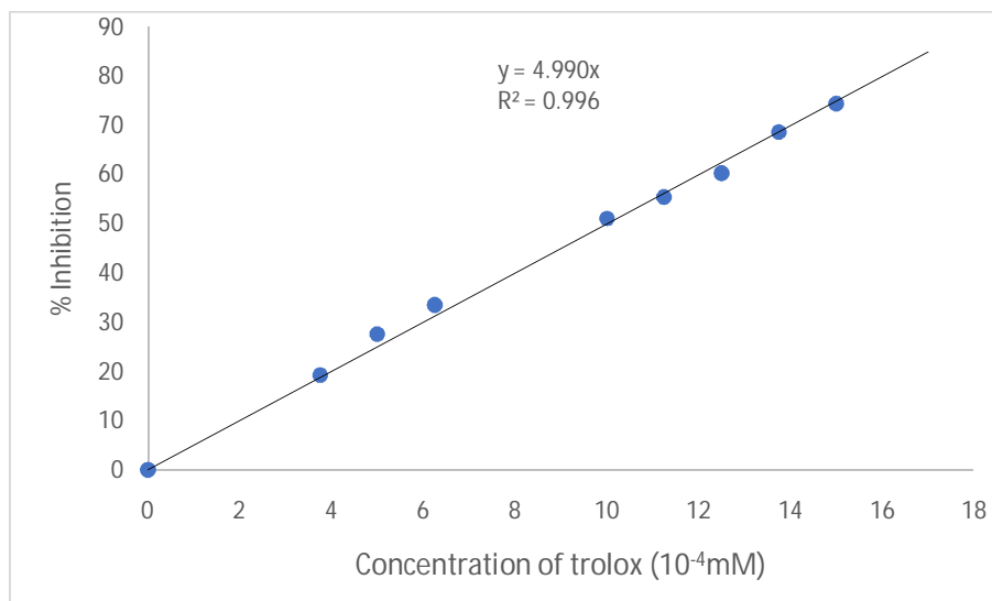
Figure 1: Trolox calibration curve for antioxidant activity assay
