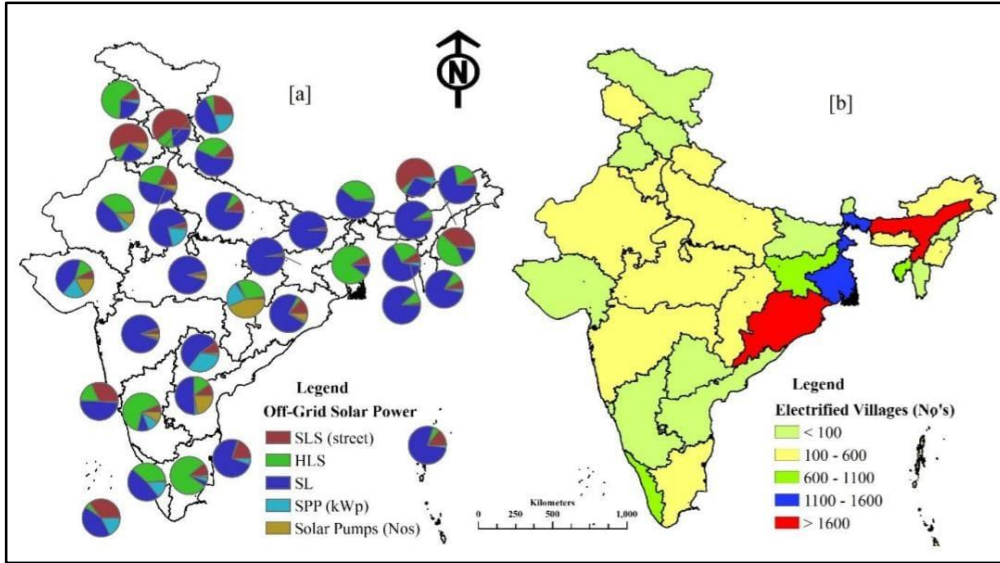
Fig. 8: [a] Displays the capacity of off-grid solar power (SLS, HLS, SL, SPPs, and Solar Pumps) state wise, and [b] Displays the number of state-level electrified villages achieved using off-grid solar power as of March 30, 2021, based on MNRE data that is currently available.
