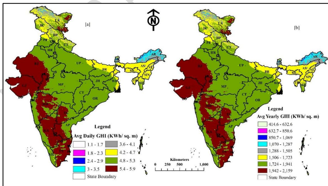
Fig. 6: [a] Illustrates the average daily Global Horizontal Irradiation (GHI) in kWh/m 2 , and [b] illustrates the average annual Global Horizontal Irradiation (GHI) in kWh/m 2 .
