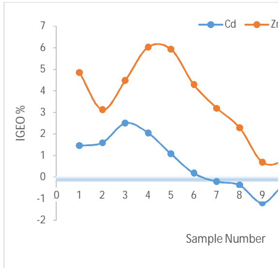
Fig. 6. The igeo values distribution for the heavy metals for the studied samples
