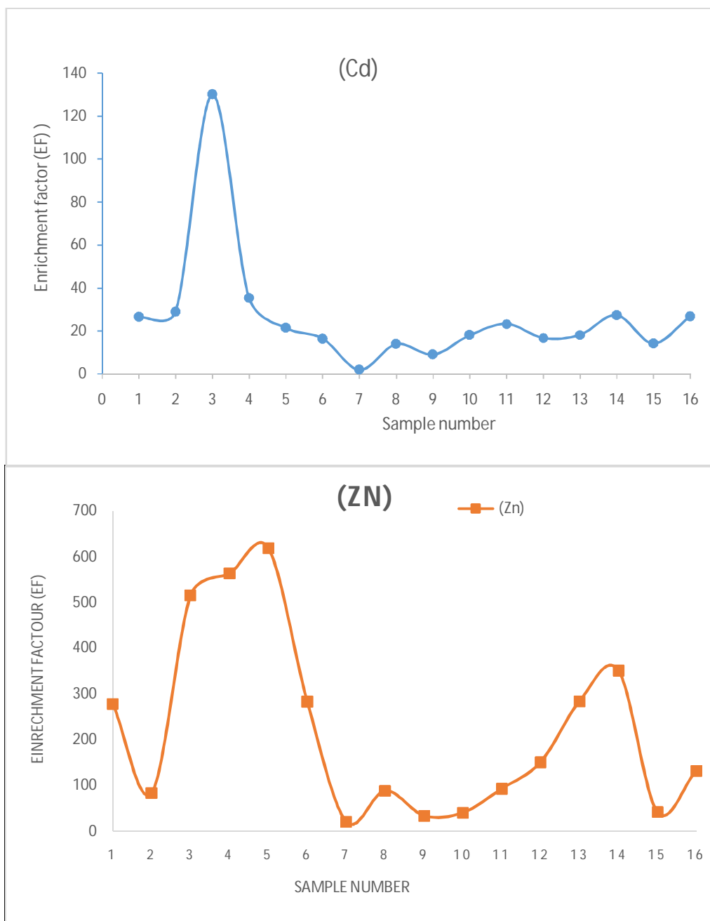
Fig. 5. The Enrichment Factor (EF) distribution for Cd and Zn of the study samples
