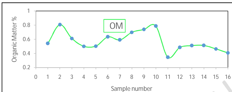
Fig.:4 Distribution of metal concentration (ppm) for Cd, Fe, Zn, Cu, Pb, and Mn and percentage of organic matter (OM%) and CaOwt% for the surfaces sediment samples from Wadi Al-Wala area.
