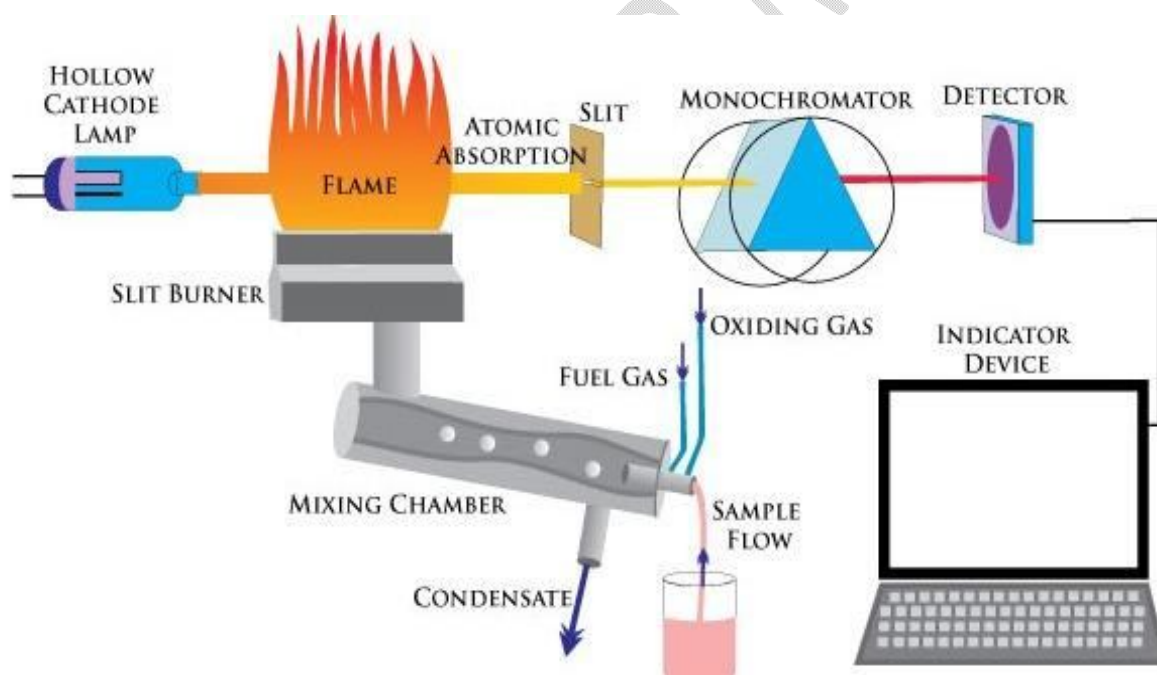
Figure 7: The principle of AAS instrumentation (Robert and Gustav 2018)
