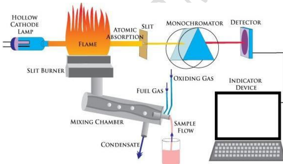
Figure 7: The principle of AAS instrumentation
