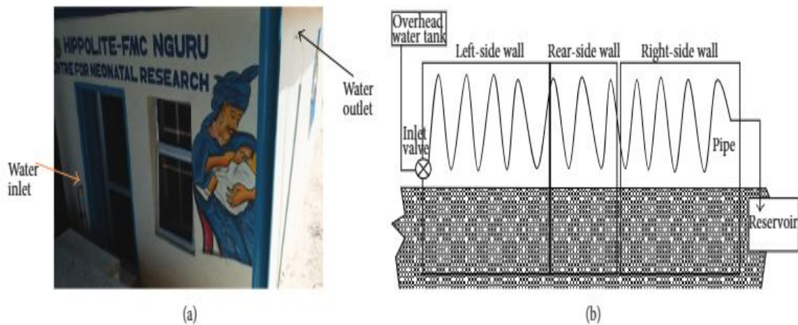
FIGURE 2: (a) Lab-1 showing heat exchanger water inlet and outlet. (b) Heat exchanger copper piping through the walls of Lab-1. Overhead tank delivered water through an inlet valve. Circulation was ensured automatically through the positive pressure head created by the relative height of the overhead tank. Cool water in the under-surface reservoir was pumped back to overhead tank when required.
