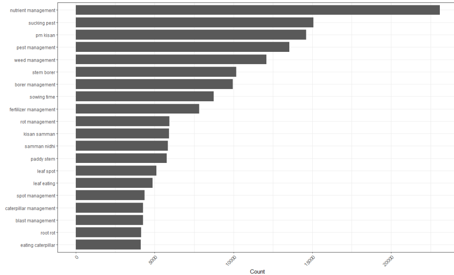
Fig5 Top 20 bigrams appearing in the farmers' queries
