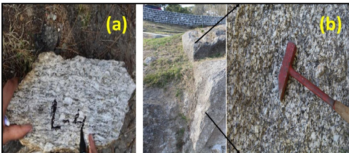
Figure 5. (a) Augen gneiss, (b) Granite
