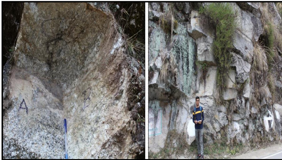
Figure 9. Three sets of joints
