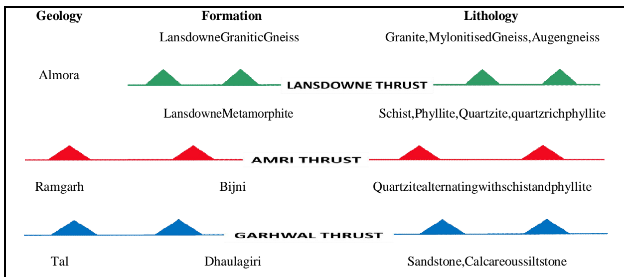
Fig 3. Litho-tectonic succession in the Lansdowne area [17]
