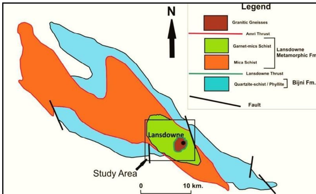
Figure 4. Geological Map of Lansdowne Area (after Fuchs and Sinha, 1978)
