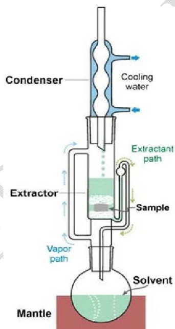
Fig.1: Parts of Soxhlet
