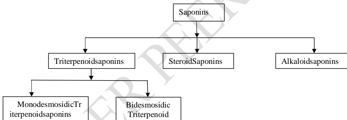
Figure 2: Categories of saponins.
