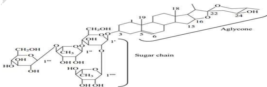
Figure 3: The chemical structure of steroid saponin.
