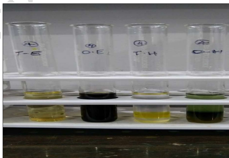
Fig.11: Test for cardiac glycosides
