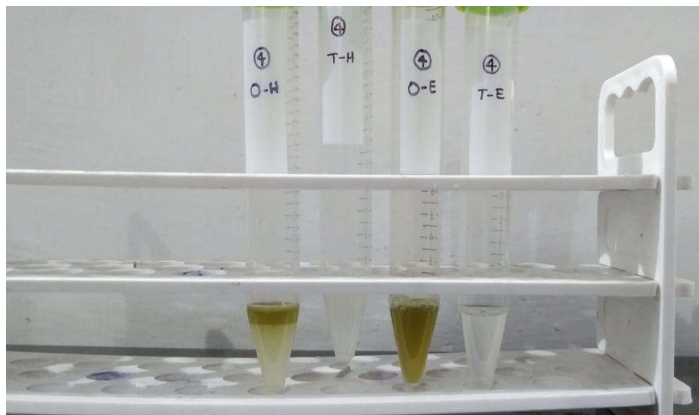
Fig.4: Test for saponins (Frothing test)
