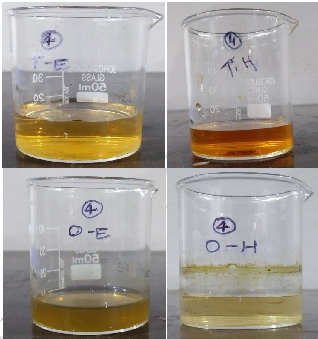
Fig.12: Test for tannins
