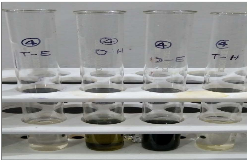
Fig.8: Test for terpenoids (Salkowski's test):
