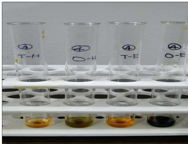
Fig.6: Test for Phenolics
