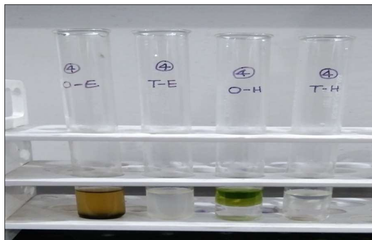
Fig.13: Test for steroids (Lieberman-Burchard test)
