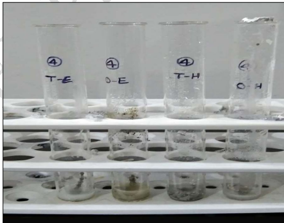
Fig.5: Test for Flavonoids (Cyanidine test)
