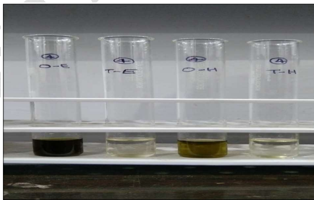
Fig.7: Test for amino acids and proteins (1% ninhydrin solution)
