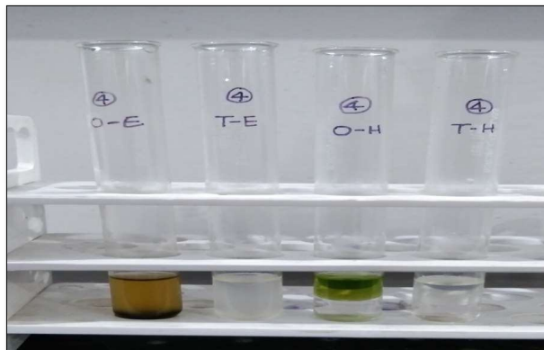
Fig.13: Test for steroids (Lieberman-Burchard test)
