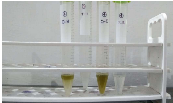
Fig.4: Test for saponins (Frothing test)
