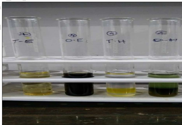
Fig.11: Test for cardiac glycosides
