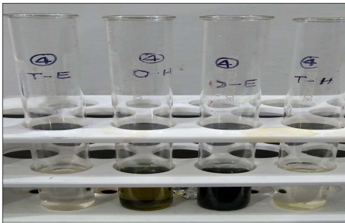
Fig.8: Test for terpenoids (Salkowski's test):
