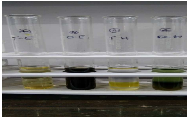
Fig.10: Test for carbohydrates (Benedict's test)
