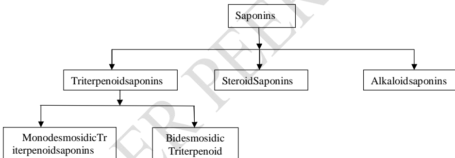
Figure 1: Categories of saponins.
