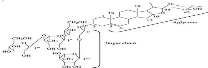
Figure 2: The chemical structure of steroid saponin.
