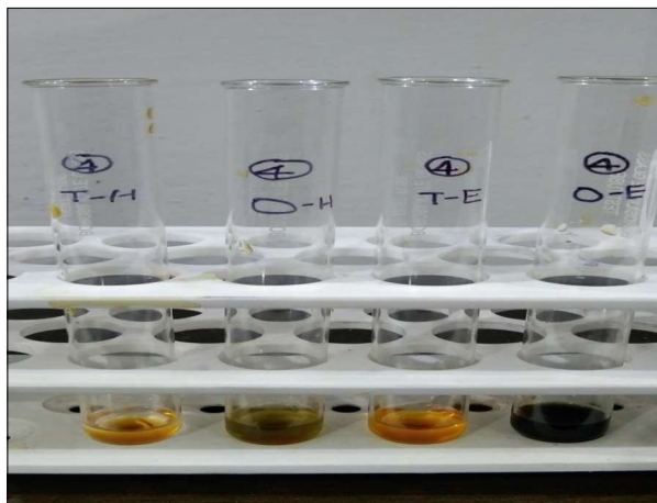
Fig.6: Test for Phenolics
