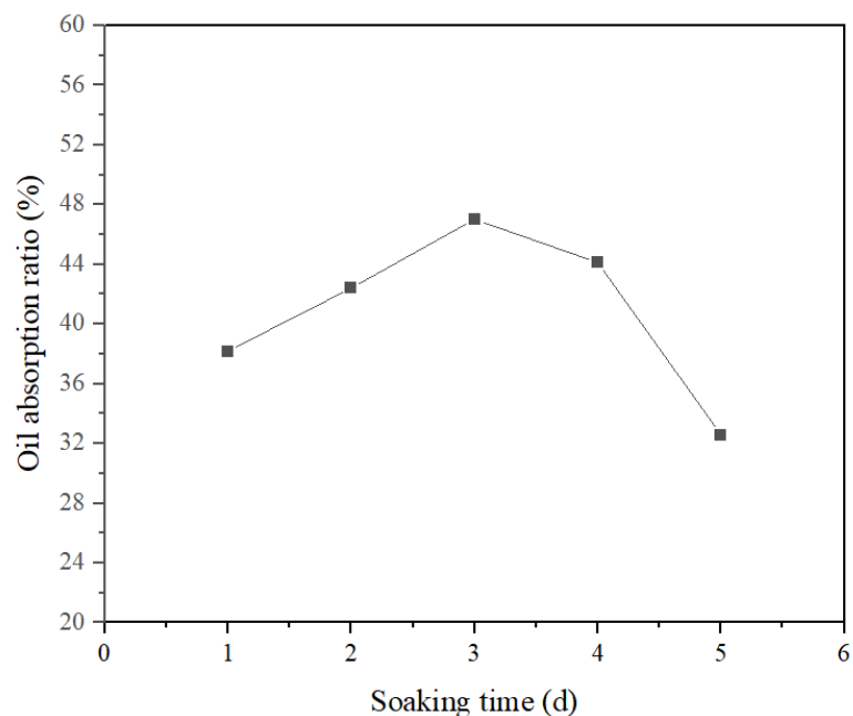
Fig 1 Relationship between fiber oil absorption rate and soaking time
