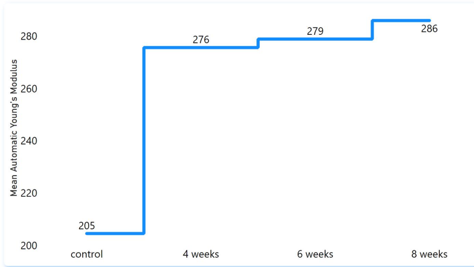
Figure 10. Mean Young's modulus
