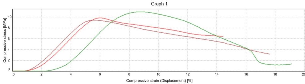
Figure 6. Control stress-displacement graph
