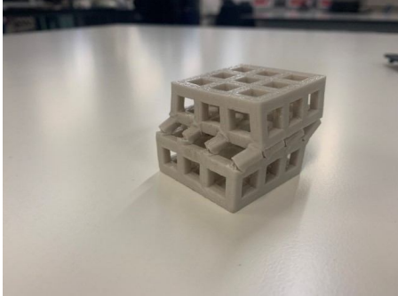
Figure 5. Deformation of a compressed 3D lattice structure
