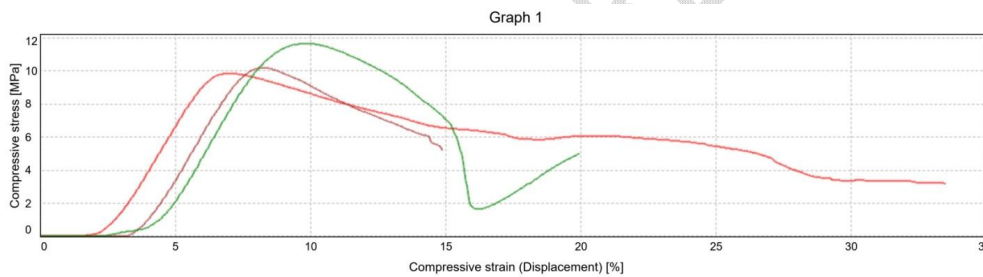
Figure 8. 6-week stress-displacement graph
