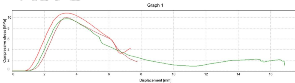
Figure 7. 4-week stress-displacement graph
