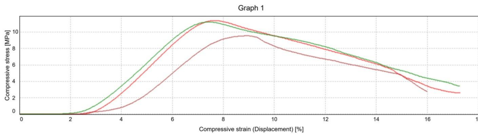
Figure 9. 8-week stress-displacement graph
