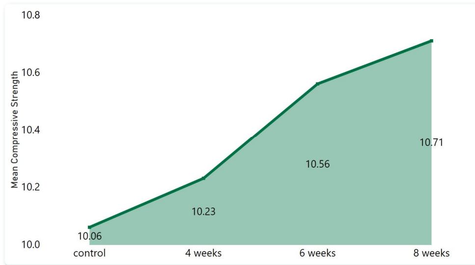
Figure 11. Mean compressive strength
