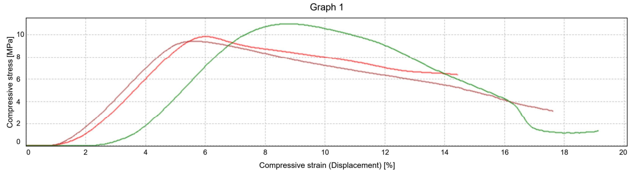
Figure 6. Control stress-displacement graph
