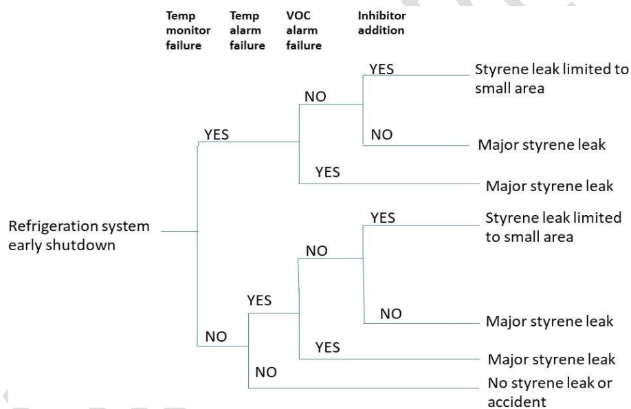
Fig.7 Event Tree Analysis for Refrigeration System Shutdown
