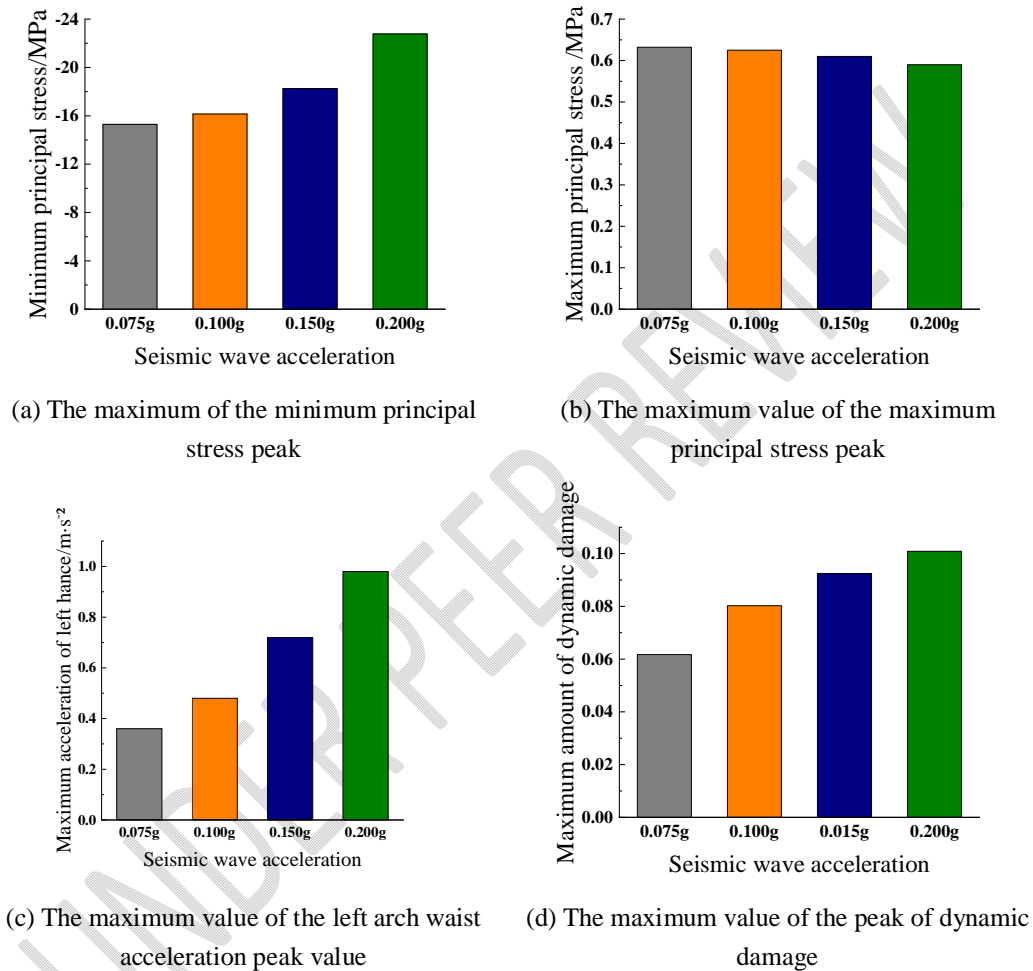
Fig. 7 The pattern of maximum dynamic response and maximum dynamic damage quantity with varying seismic wave intensity.
