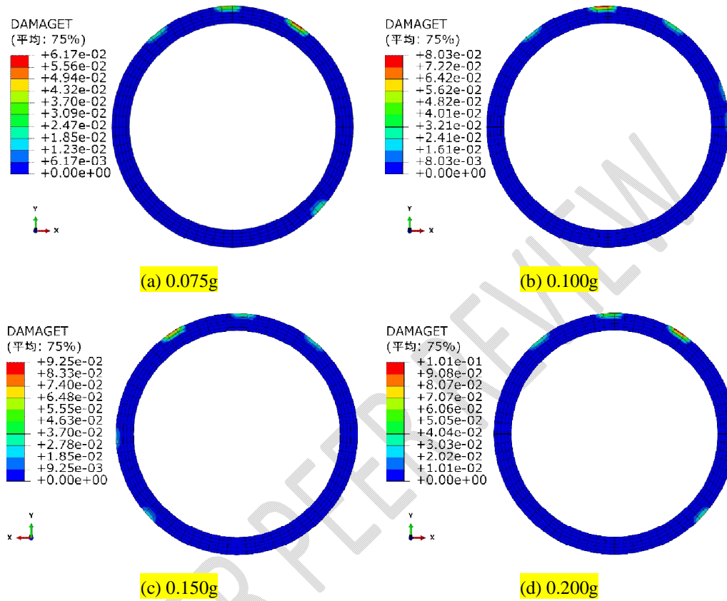
Fig. 8 Distribution of dynamic damage quantity in the lining structure under different seismic wave intensities.
