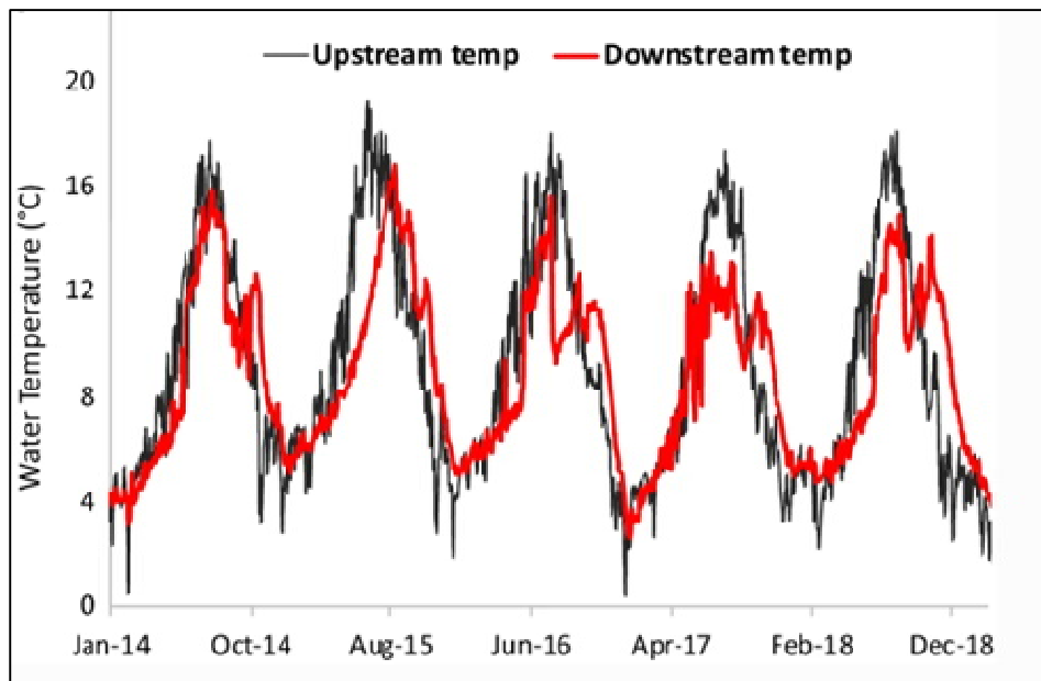
Figure 2: Shows the temperature variation of downstream and upstream through the year of Detroit dam in the USA (Ahmad et al., 2020)
