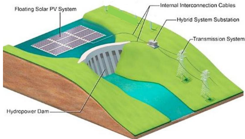
Figure 8: Schematic diagram of Float solar PV with hydropower.
