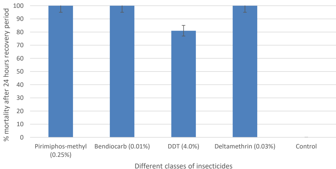
Figure 2: Mortality rate of C. quinquefasciatus to different insecticide classes
