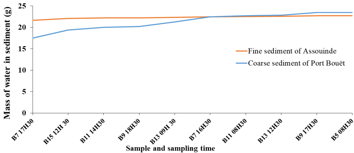
Fig 6: Water mass for saturation of 10 samples of 100 g of fine sediment from Assouindé and coarse sediment from Port Bouët.
