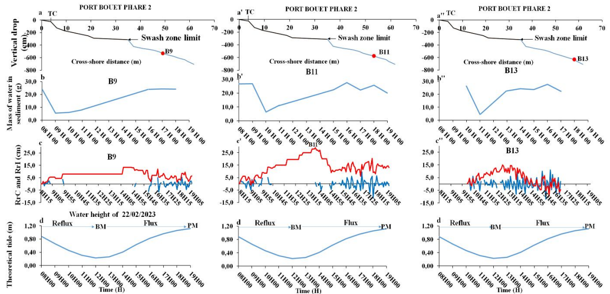
Fig 5: Relationship between sediment water content and morphology of a point on the foreshore during a tidal cycle in a coarse sand facies.
