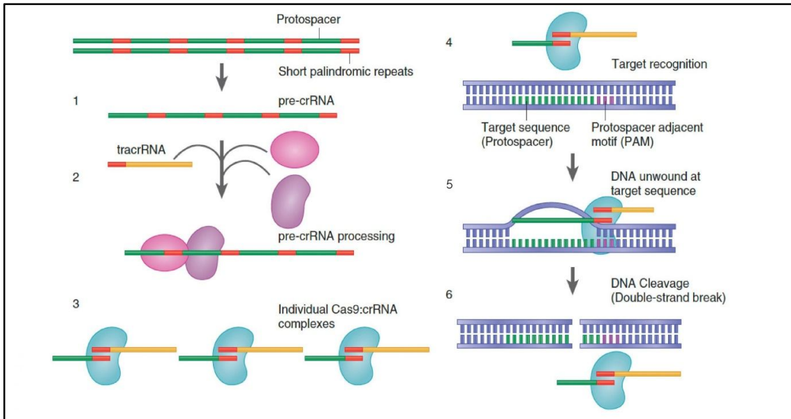
Fig. 2. Mechanisms of CRISPR/Cas Systems
