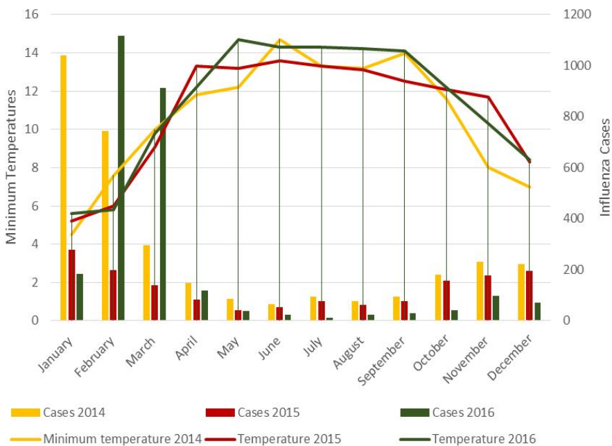
Figure 2. Influenza cases and minimum temperatures reported in Hidalgo 2014-2016
