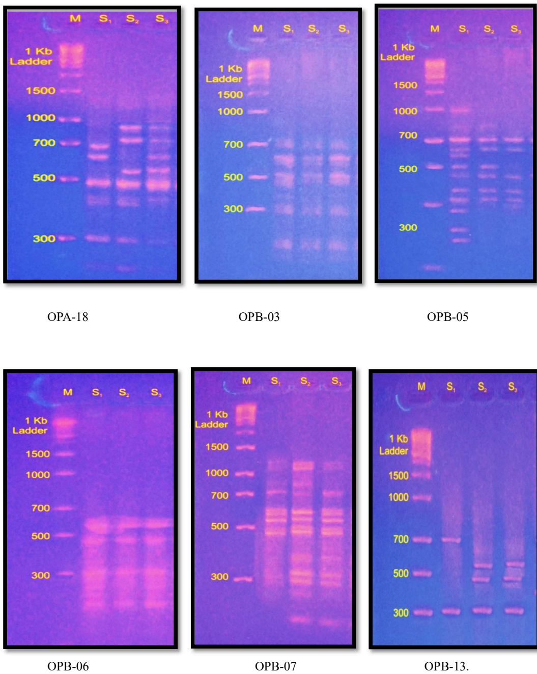
Figure 1: Agarose gels showing polymorphic and monomorphic primers (OPA-01, OPA-02, OPA-04, OPA-09, OPA-13, OPA -15, OPA-18, OPB-03, OPB-05, OPB-06, OPB-07, 0OPB-13).
