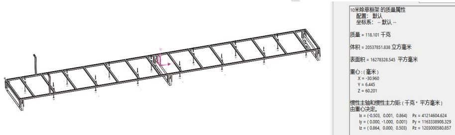
Figure 10. Center of gravity and mass of the overall frame
