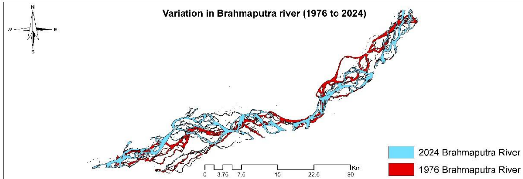
Fig.4. Morphology of Brahmaputra river from 1976 to 2024
