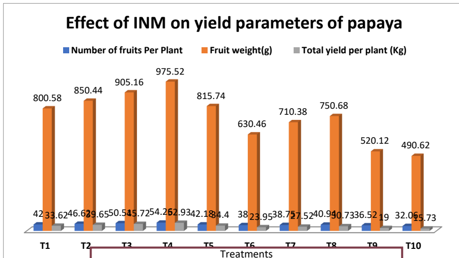
Fig.1. Effect of INM on yield parameters of papaya
