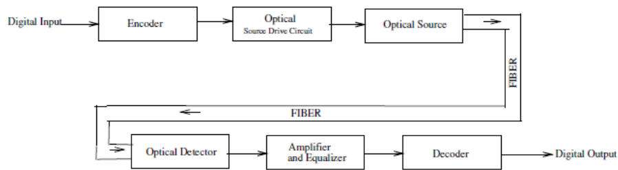
Figure 1: A simple block diagram of digital communication through an optical fiber
