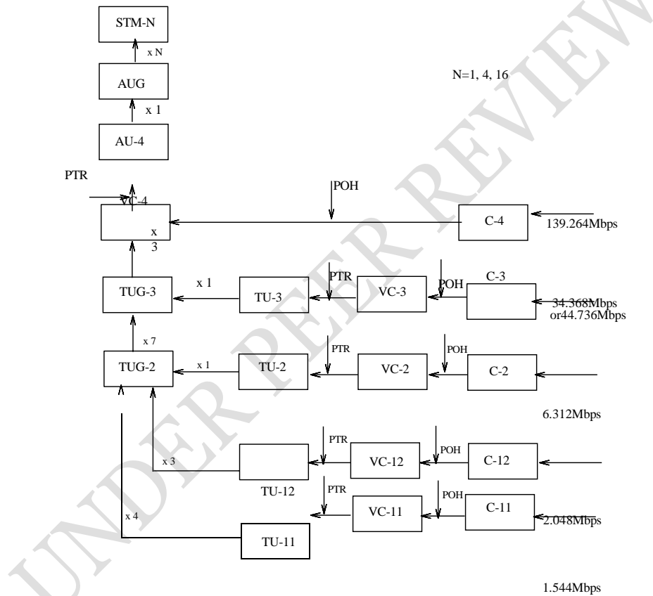
Figure 5: Multiplexing tree for SDH
