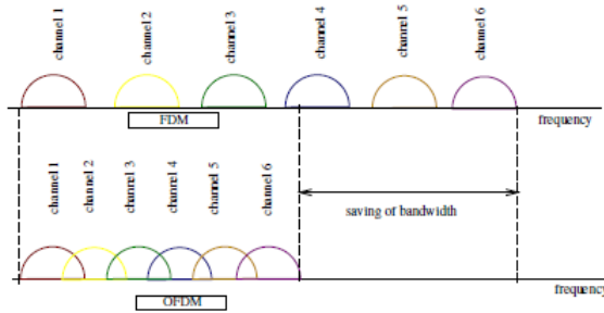
Figure11: Comparison of FDM and OFDM to illustrate bandwidth saving
