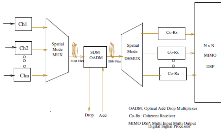
Figure 17: SDM transmission system
