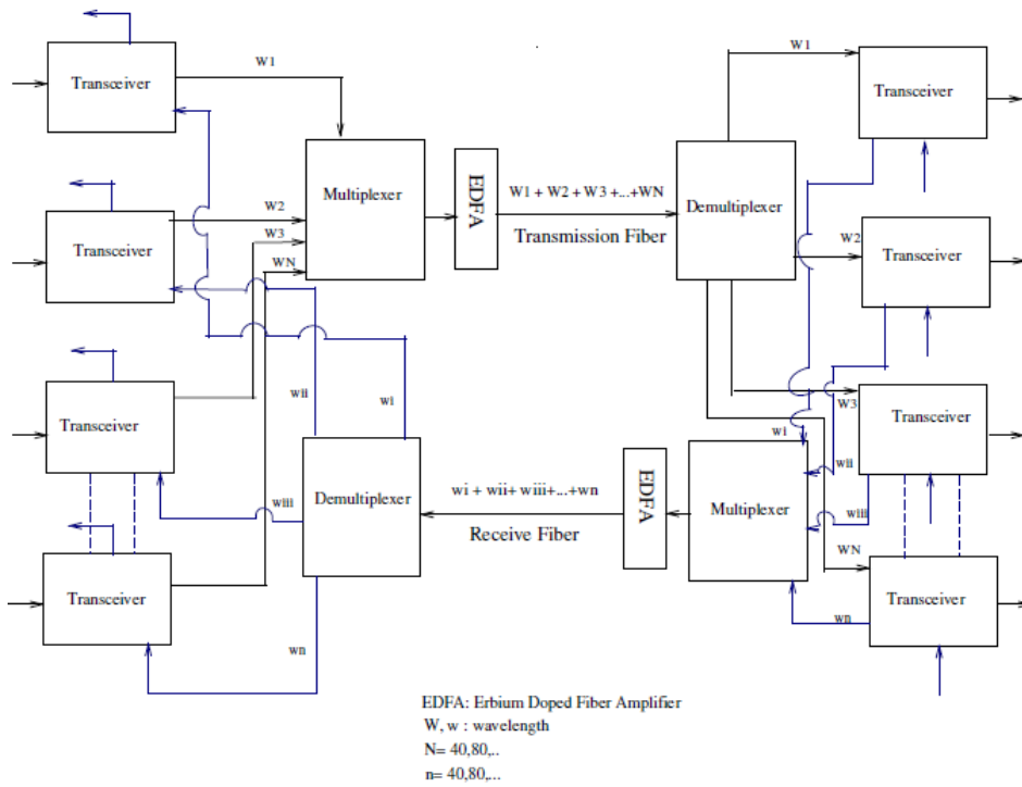
Figure 9: A simple block diagram of a DWDM system
