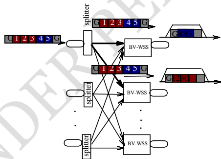
Figure 14: Broadcast and Select Architecture
