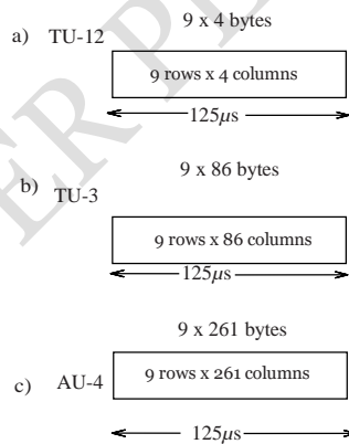
Figure 8: Frame structure of different SDH multiplexing stages
