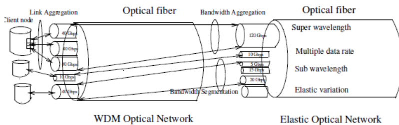
Figure 15: Difference between WDM optical networks and EONs
