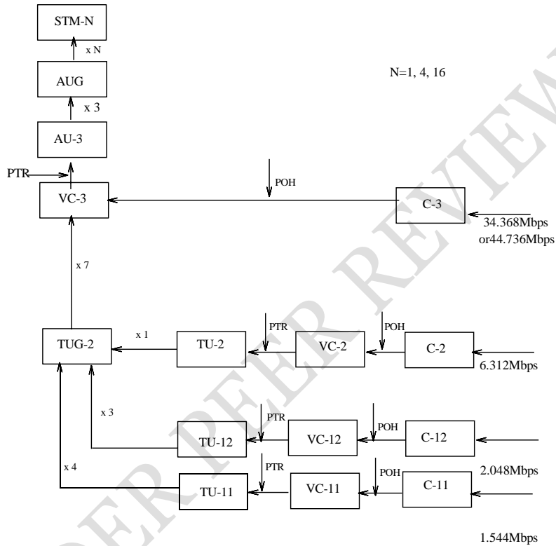
Figure 6: Multiplexing tree (alternate path) for SDH
