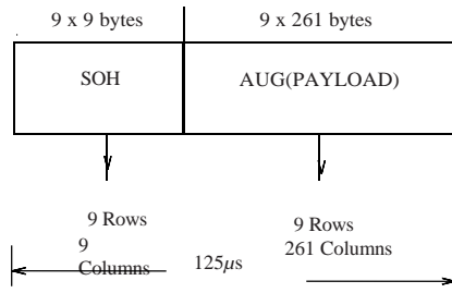
Figure 7: STM-1Frame
