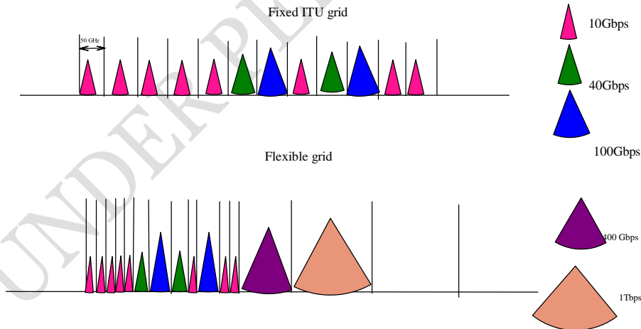
Figure 12: Comparison of spectral widths in fixed and flexible grid optical networks
