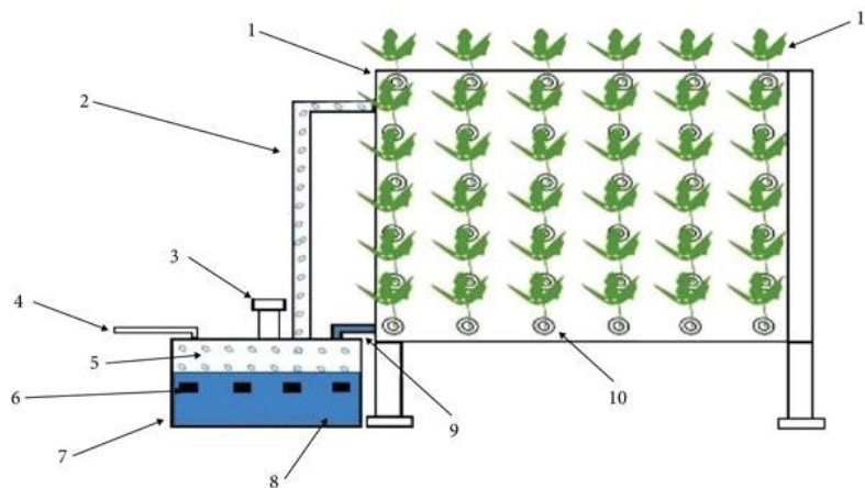
Fig. 1. Schematic representation of an aeroponic system in vertical farming
