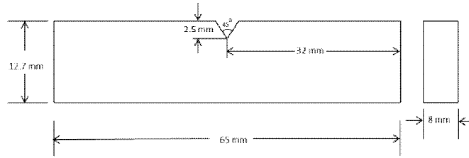
Figure 4: Specimen geometry of the Impact test (6)
