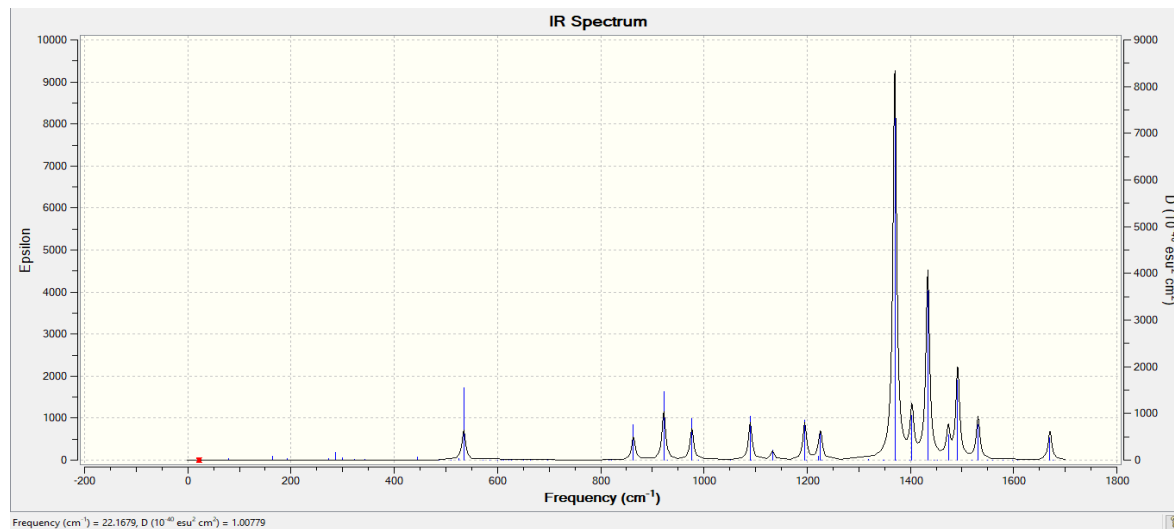
Figure 2b: Anionic perfluoropentacene (B3LYP/6-31+G (d))
