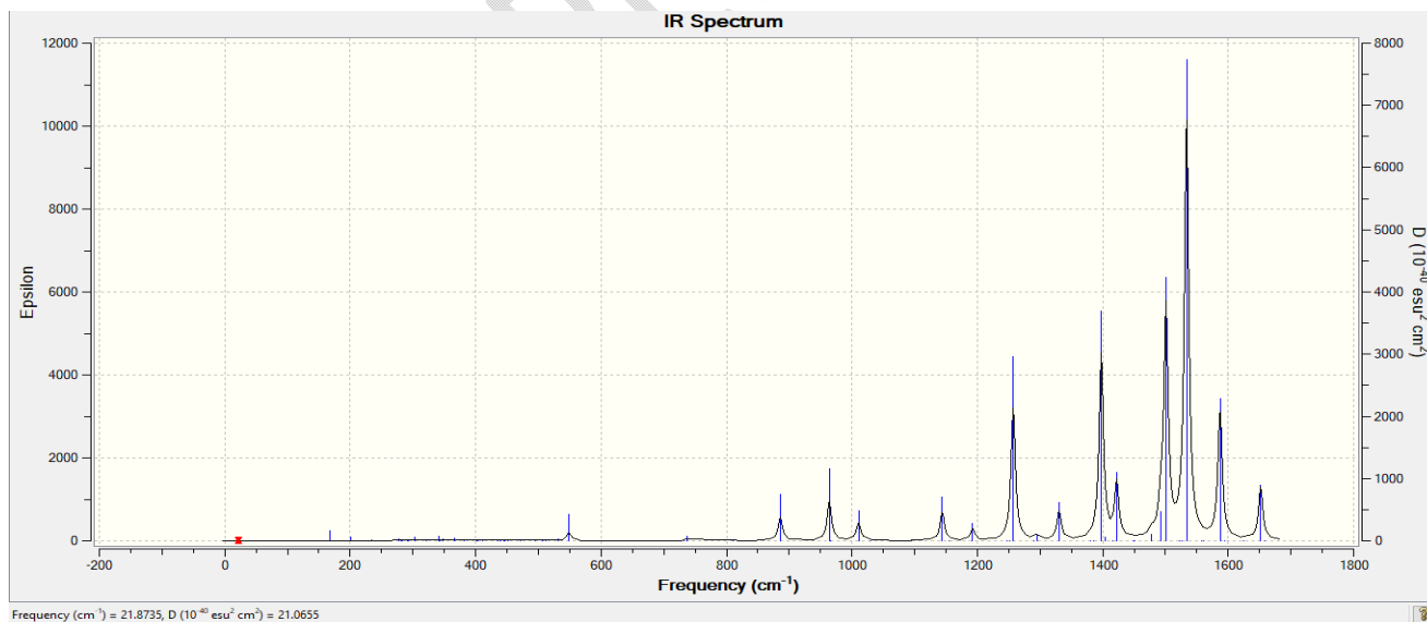
Figure 2c: Cationic perfluoropentacene (B3LYP/6-31+G (d))
