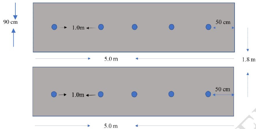
Figure 2. Layout of an individual plot
