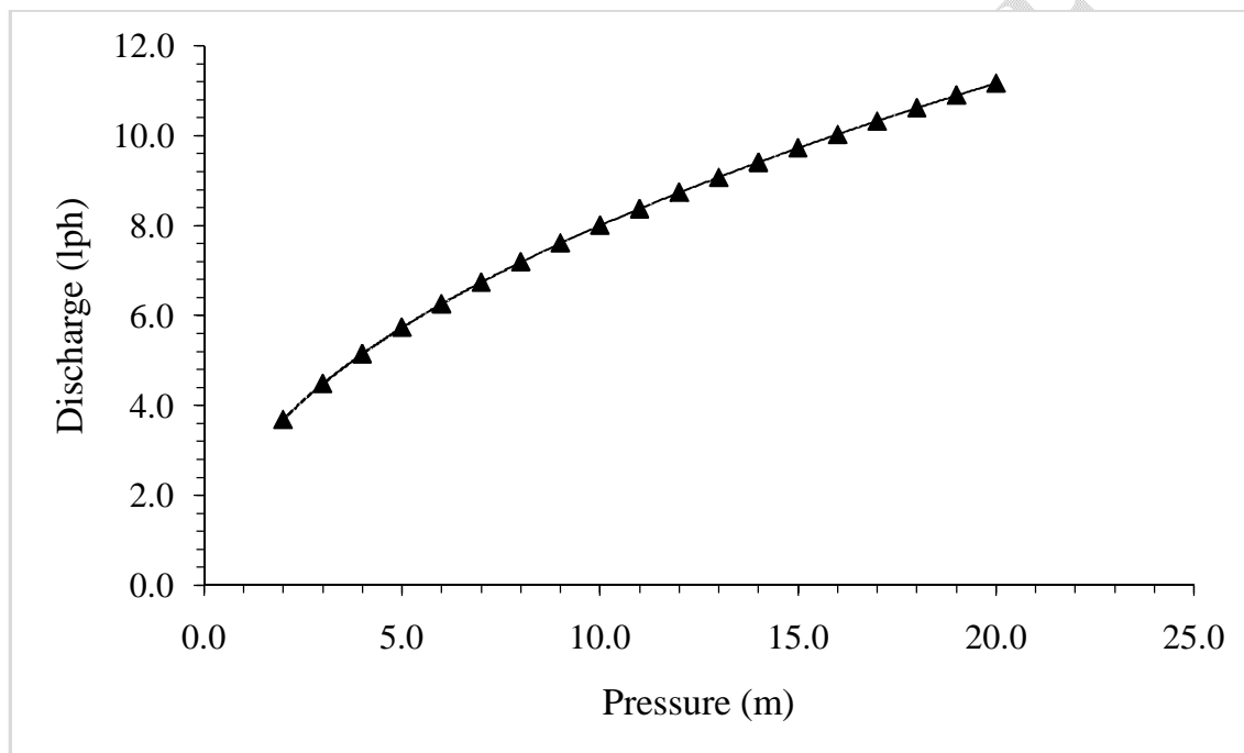
Fig. 2 Pressure Discharge Relationship Curve
