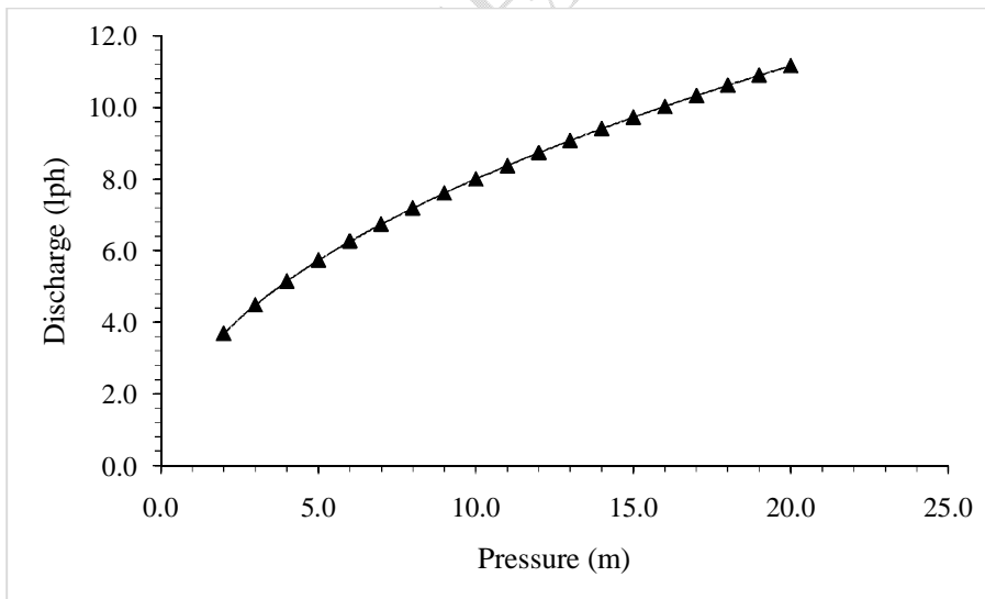
Fig. 1 Pressure Discharge Relationship Curve
