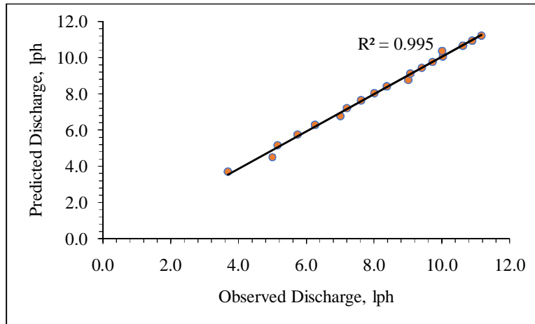
Fig. 2 Observed and Predicted Emitter Flow Rate
