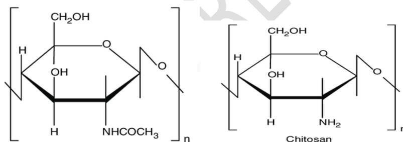
Fig. 2. Chemical structure of chitin and chitosan
