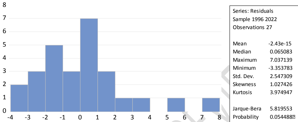
Figure 1: Normality Test
