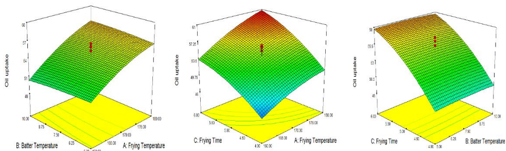
Figure 1. 3-D surface graph showing the effect of process variables on oil uptake of ghewar
