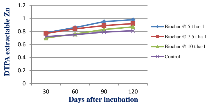
Fig 3. Effect of different levels of mulberry stalk biochar on DTPA extractable iron, manganese, zinc and copper ( \text{mg kg}^{-1} ) release during incubation period (30, 60, 90 and 120 DAI)
