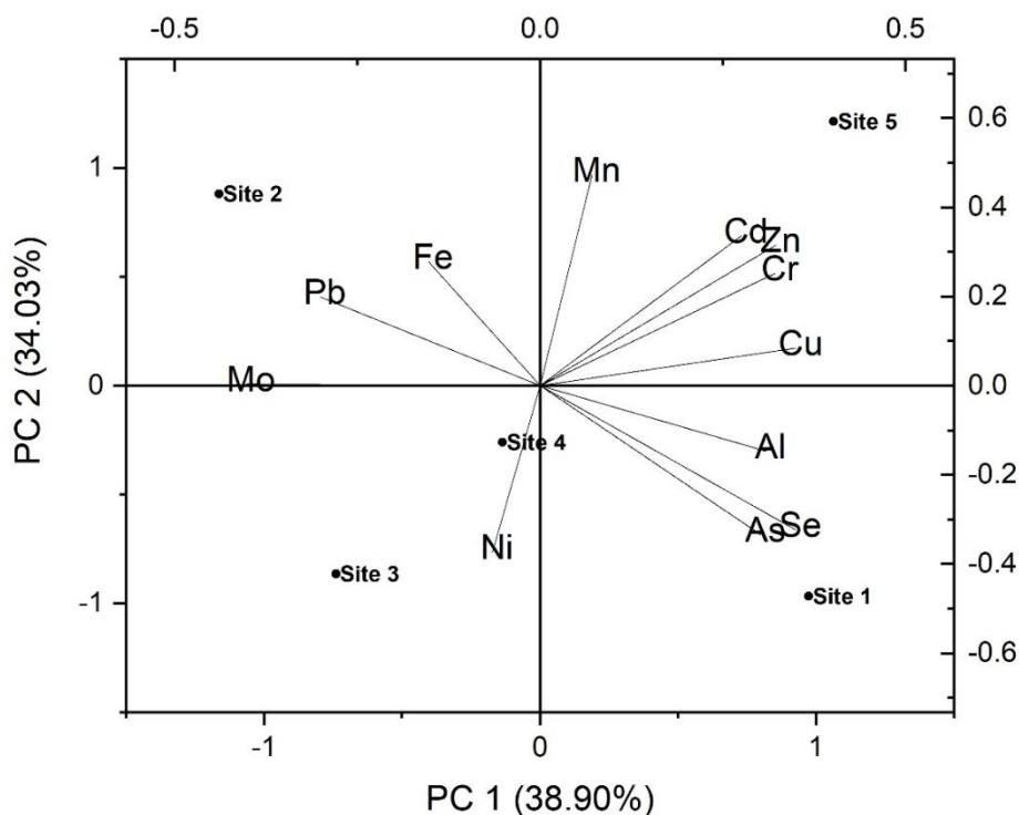
Figure 5. Principal component analysis revealing the multivariate relationships of the heavy metals of the study sites
