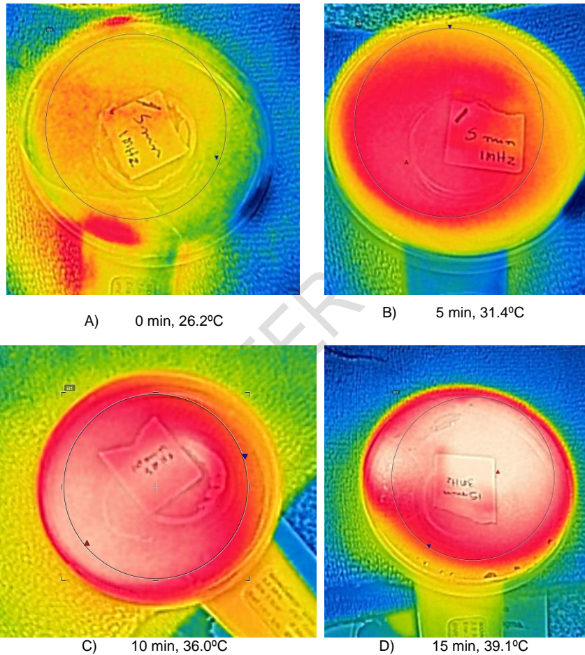
Figure 3: Thermography Images of the plates. Acquisition of thermographic images of the plates: before the application of UST (Control) and after 5 minutes, 10 minutes and 15 minutes. The images are illustrative, and the results are the simple average of the temperature of each plate after the application of the UST.
