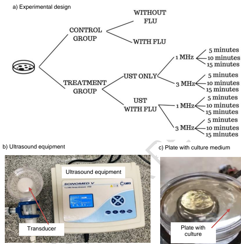
Fig 1. a) Experimental design of groups (Canva). b) Ultrasound equipment (model Sonomed V, CARCI, frequencies 1 MHz and 3 MHz), with transducer and plate without culture medium with water-based coupling gel. c) Application of ultrasound in liquid culture medium (Sabouraud Dextrose broth), Source: Personal archive.
