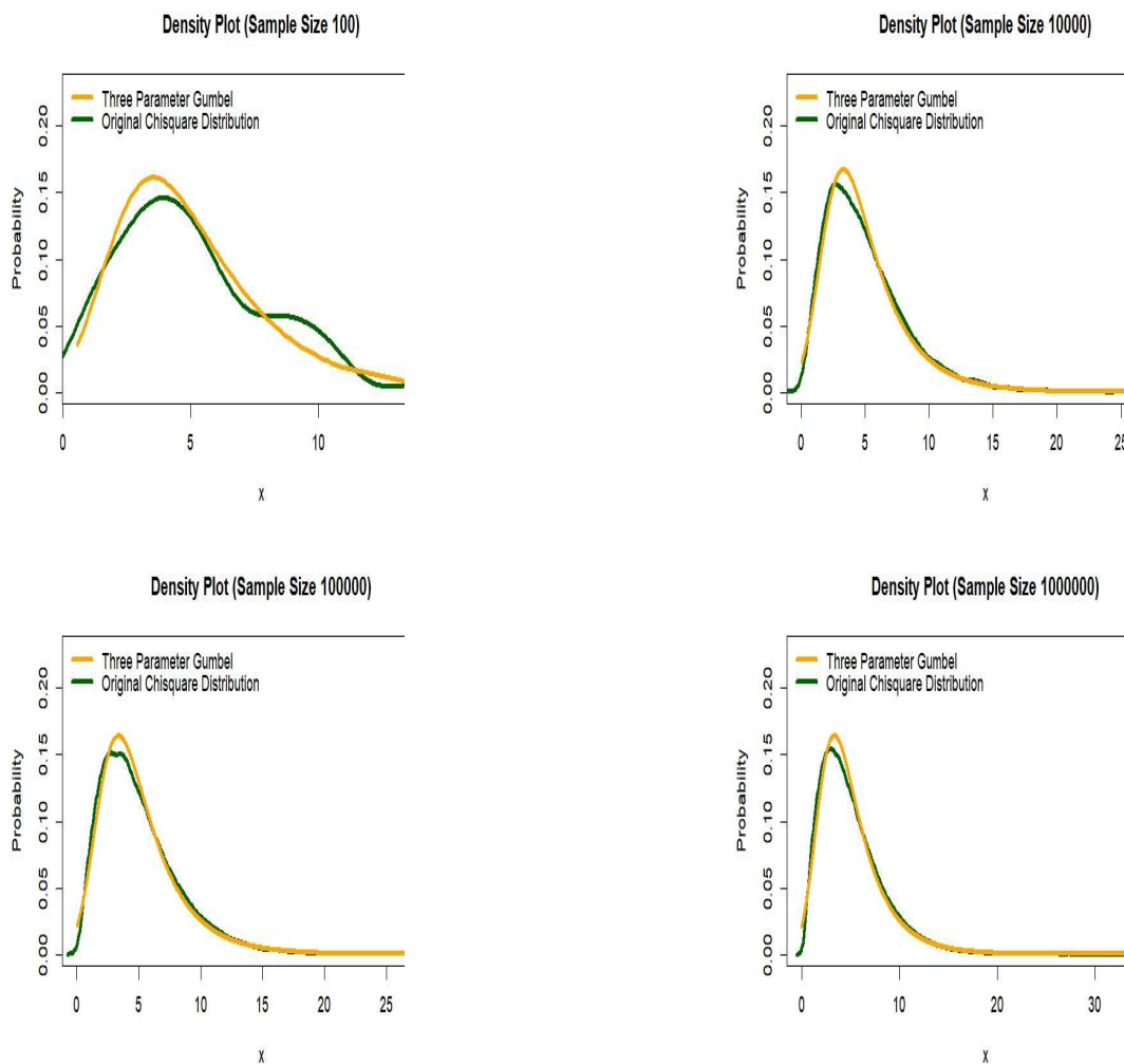
Figure 9. Asymptotic distributions for three parameters Gumbel and chi-square distributions
