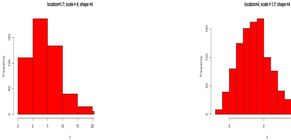
Figure 3. Distributions when \delta are n are constant
