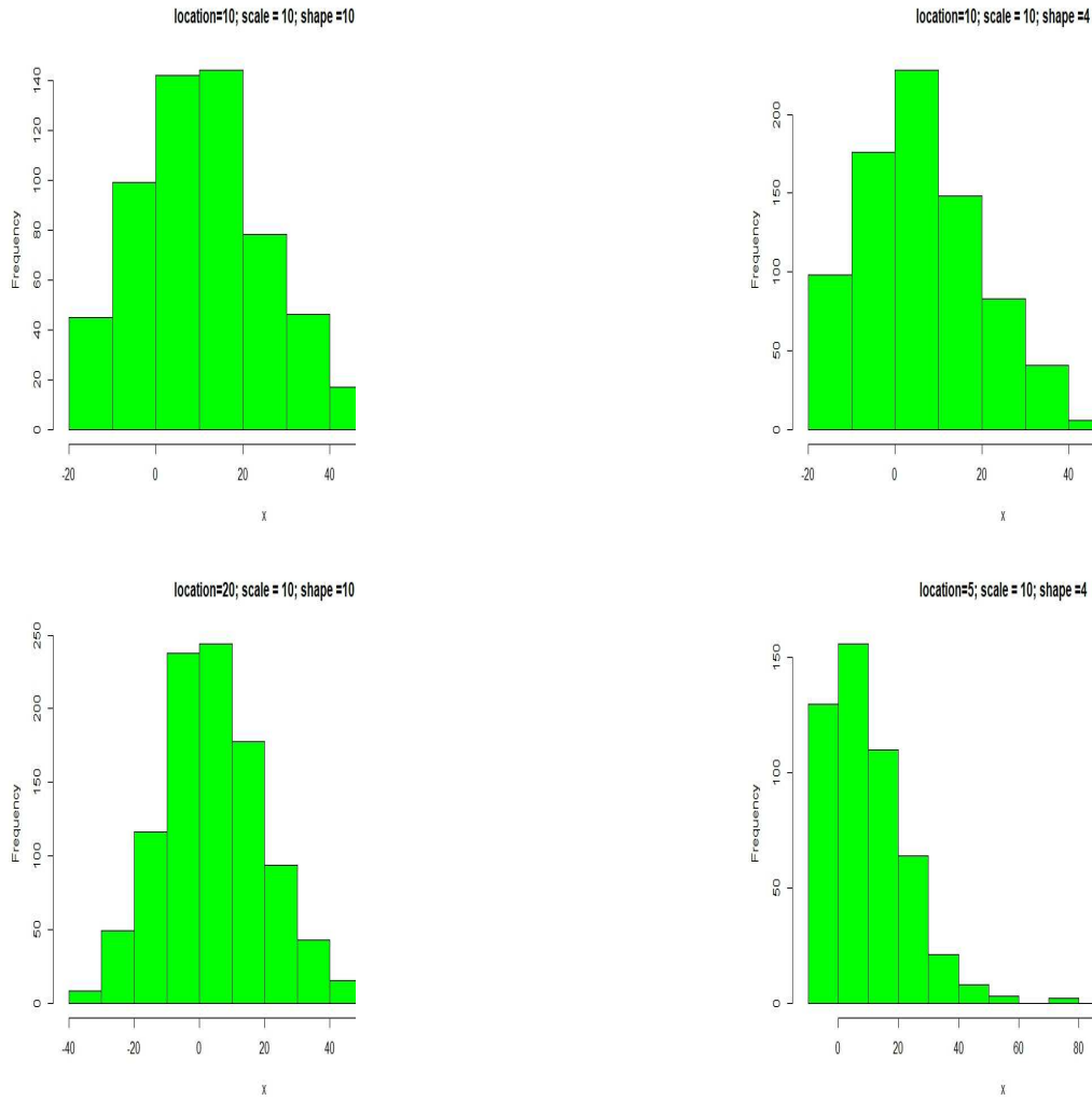
Figure 2. Distributions when \tau and n are constant
