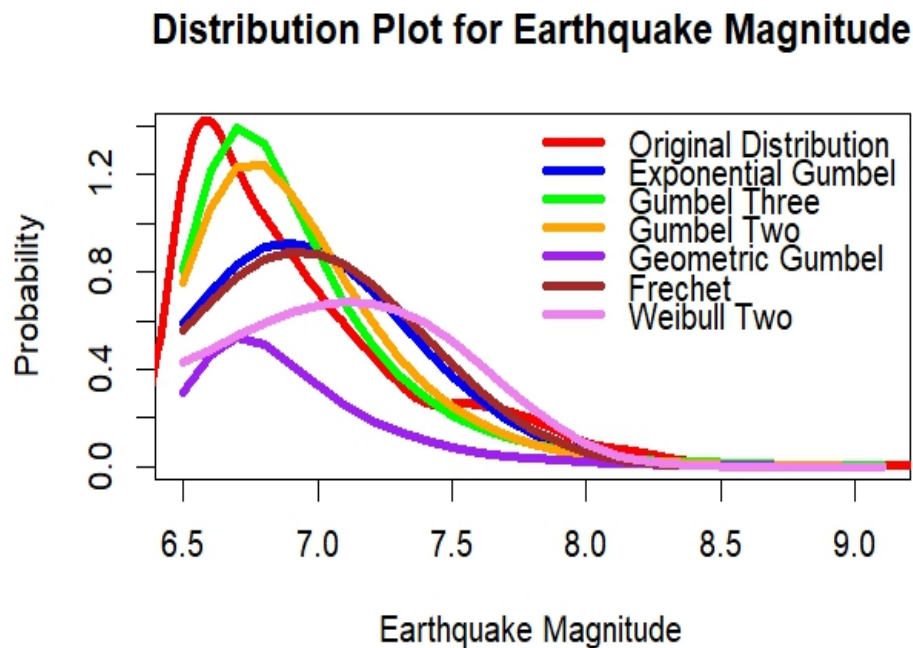
Figure 11. Data 1:Earthquake magnitude
