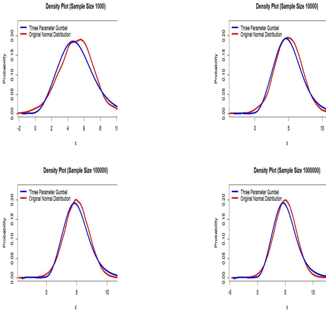
Figure 8. Asymptotic distributions for three parameters Gumbel and normal distributions
