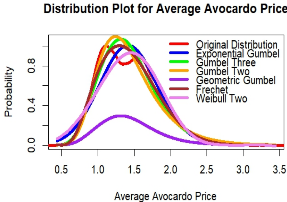
Figure 12. Data 2: Avocado prices in dollars
