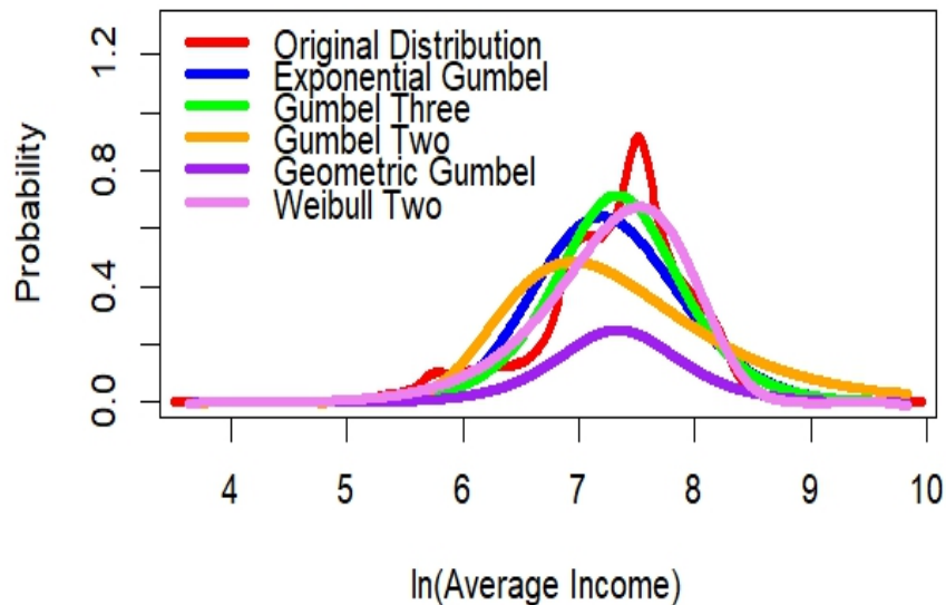
Figure 13. Income prediction data
