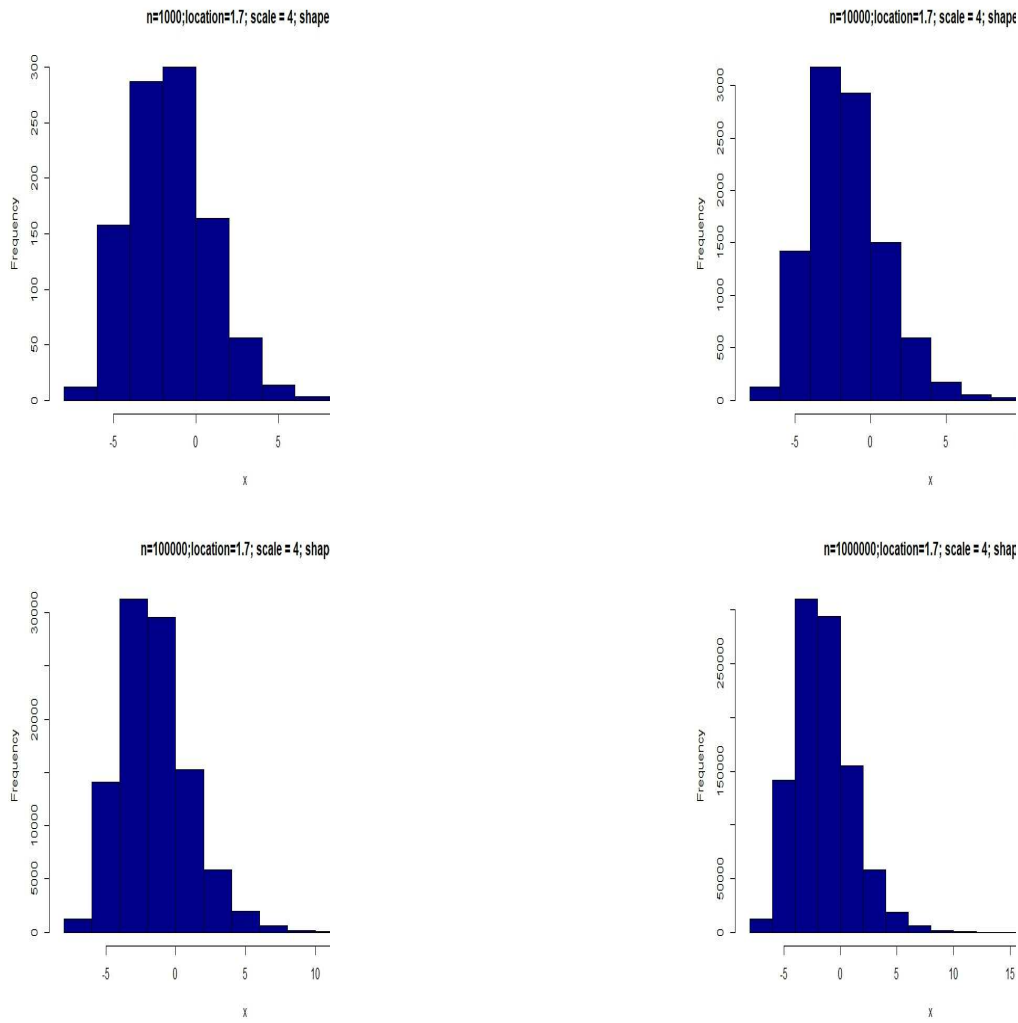
Figure 4. Distributions when \omega, \tau and \delta are constant and n is varying
