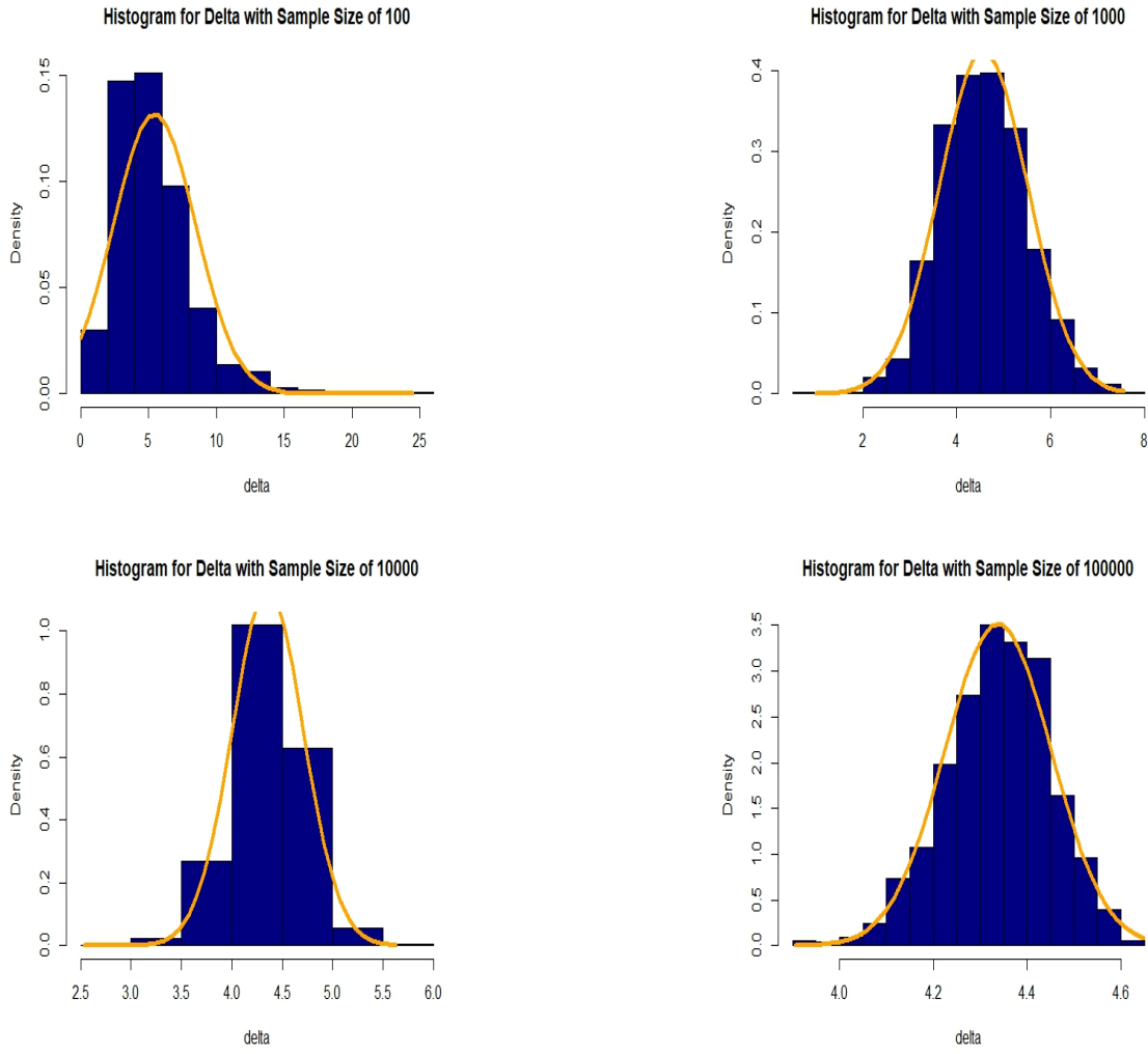
Figure 6. Asymptotic distributions for \delta
