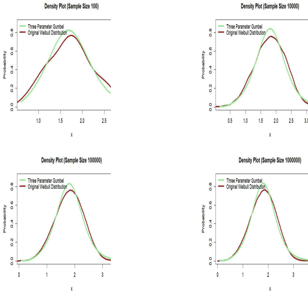
Figure 10. Asymptotic distributions for three parameters Gumbel and Weibull distributions
