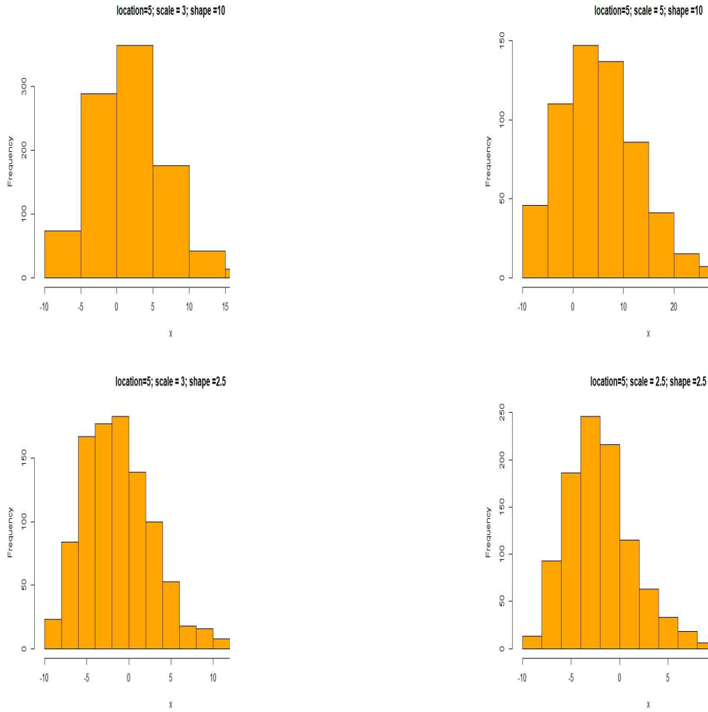
Figure 1. Distributions when \omega and n are constant
