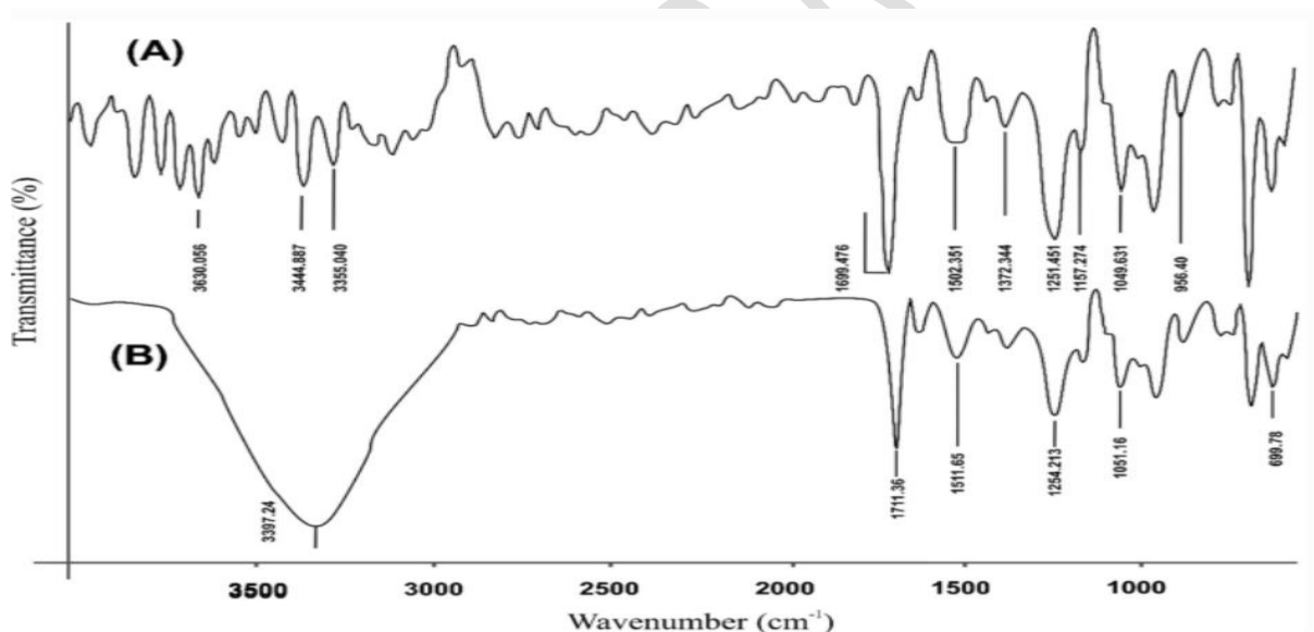
Figure 2: A) FTIR spectra of Docetaxel and B) Docetaxel polymer interaction
