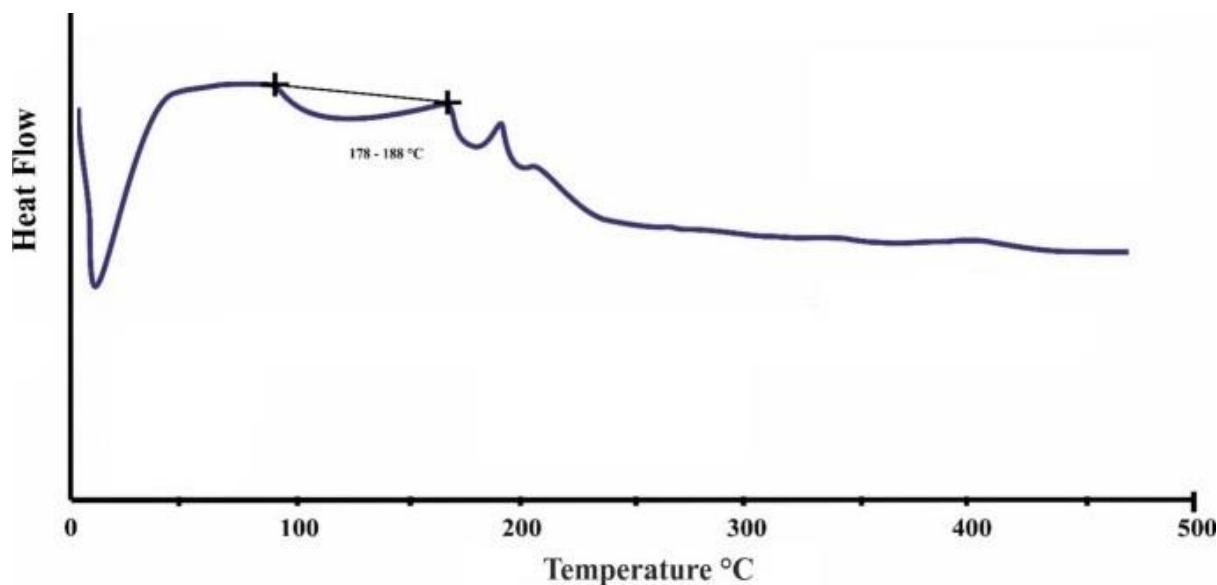
Figure 3: DSC thermograms of Docetaxel
