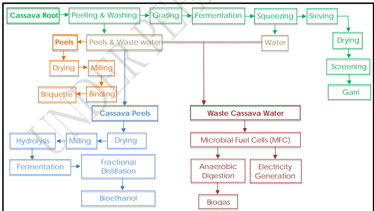
Fig. 5 Flowchart of the Garri production process, waste generated during the process, and the biofuels produced from the waste. (Adapted from
