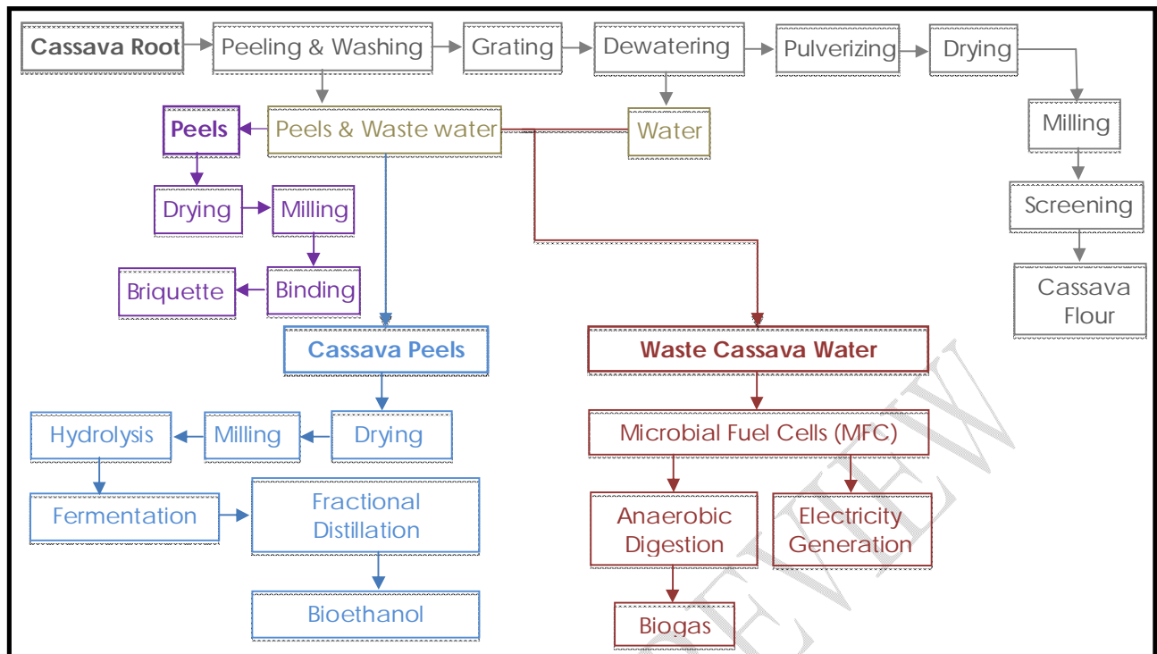
Fig. 4 Flowchart of cassava flour production process, waste generated during the process, and the biofuels produced from the waste. (Adapted from Ullah et al., 2023; Ekop et al., 2019; Siddique et al., 2017; Izah & Ohimain, 2015).
