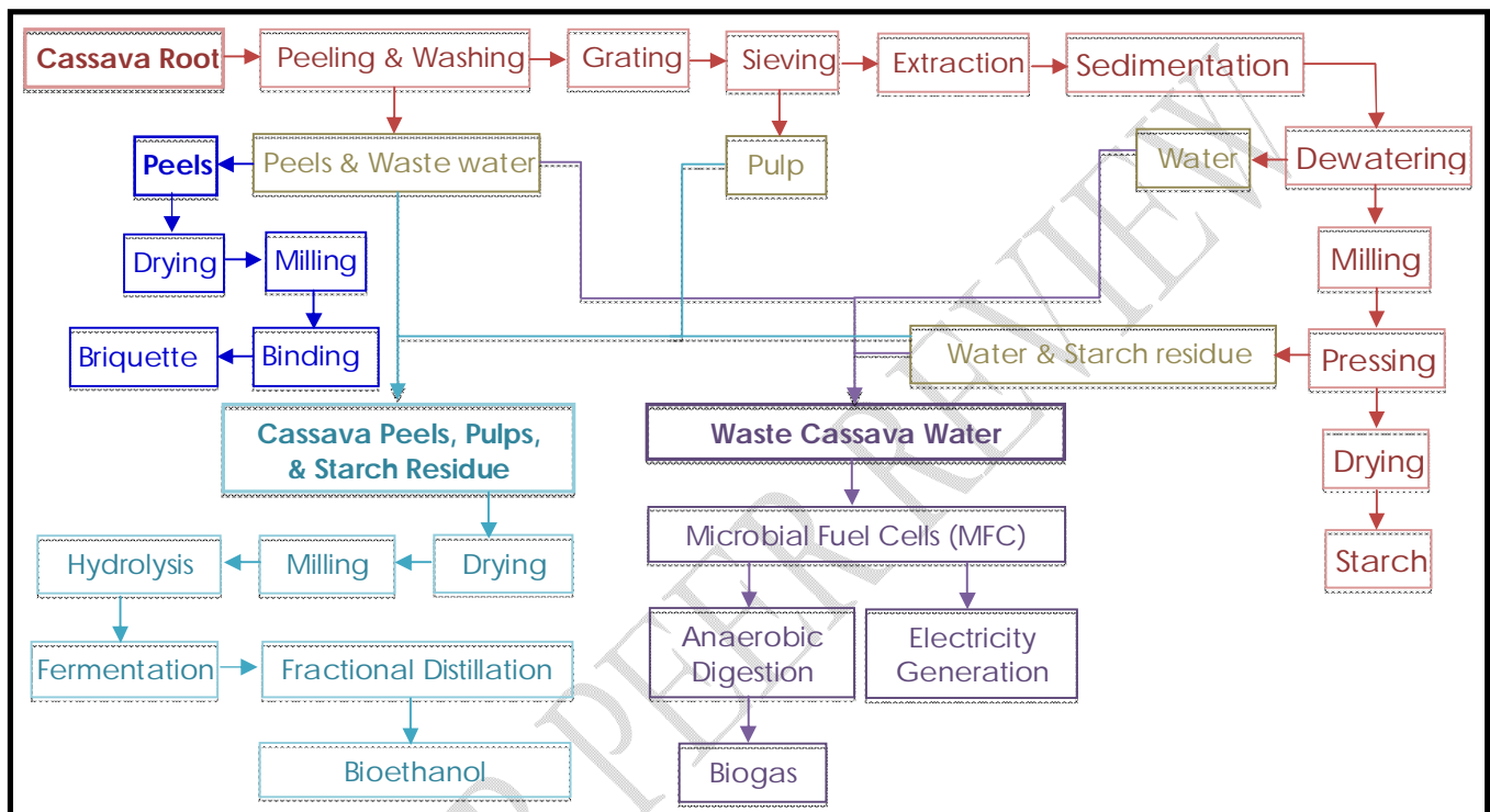
Fig. 3 Flowchart of the starch production process, waste generated during the process, and the biofuels produced from the waste. (Adapted from Ullah et al., 2023; Siddique et al., 2017; Izahand Ohimain, 2015).
