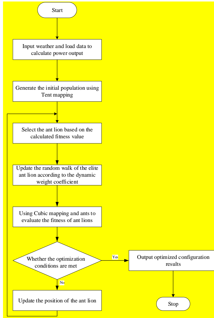
Fig. 3. Flow chart of microgrid capacity configuration based on ALO
