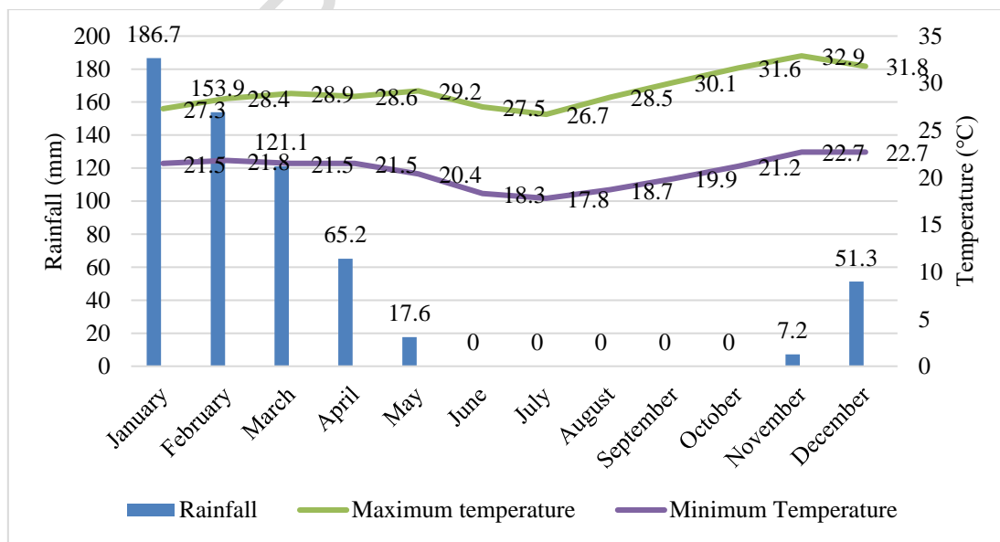
Figure 1: Climate data of the study areas from January to December in 2022.
