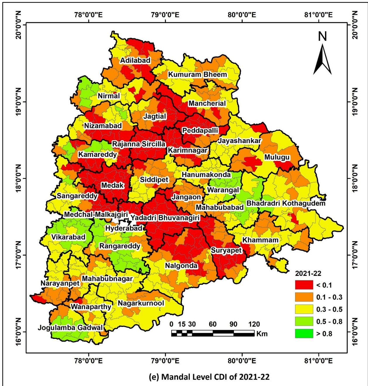
Figure6. Mandal level crop diversity index maps for 5 years (a) Mandal level CDI of 2017-18, (b) Mandal level CDI of 2018-19, (c) Mandal level CDI of 2019-20, (d) Mandal level CDI of 2020-21 and (e) Mandal level CDI of 2021-22 years.
