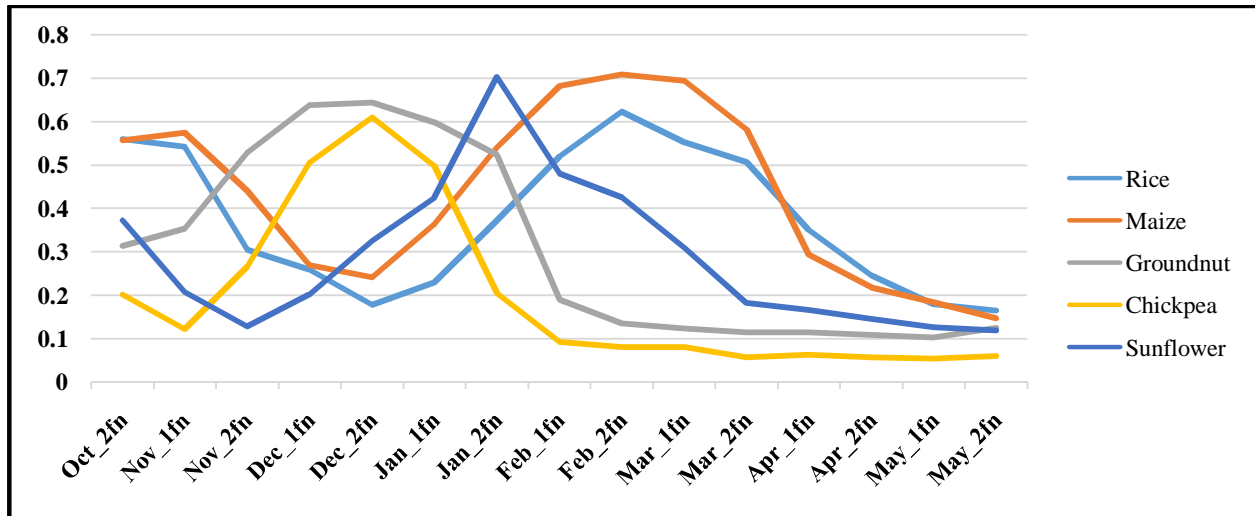
Fig 3. NDVI-based crop growth profiles for Rice, Maize, Groundnut, chickpea, and sunflower
