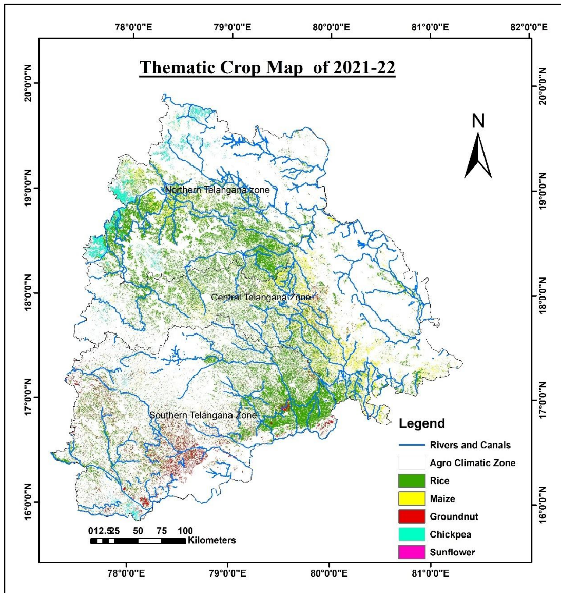
Fig 5. Crop maps of Rice, Maize, Groundnut, Chickpea, and Sunflower crops from 2017-18 to 2021-
