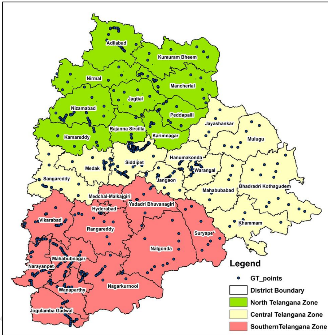
Fig 2. Study area depicting the ground truth points distribution and three agro-climatic zone
