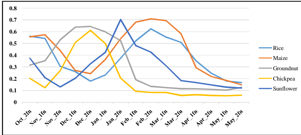
Fig III. NDVI-based crop growth profiles for Rice, Maize, Groundnut, chickpea, and sunflower
